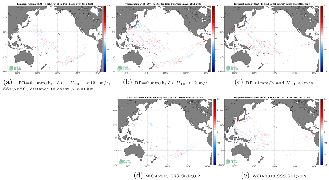
Figure 12: Temporal mean gridded over spatial boxes of size 1°x1° of \Delta SSS (SMAP SSS L4 OI v1 - 7day (IPRC) - TSG (LEGOS-DM)) for 5 different subdatasets corresponding to:RR=0 mm/h, 3 < U_{10} < 12 m/s, SST>5°C, distance to coast > 800 km (a), RR=0 mm/h, 3 < U_{10} < 12 m/s (b), RR>1mm/h and U_{10} < 4 m/s (c), WOA2013 SSS Std<0.2 (d), WOA2013 SSS Std>0.2 (e).
