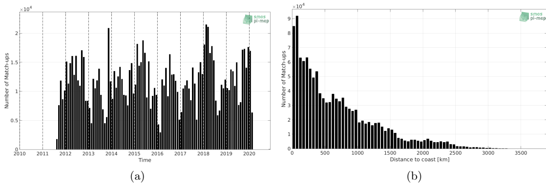
Figure 1: Number of match-ups between TSG (LEGOS-DM) and SMAP SSS L4 OI v1 - 7day (IPRC) SSS as a function of time (a) and as function of the distance to coast (b) over the Pacific Ocean Pi-MEP region and for the full satellite product period.
