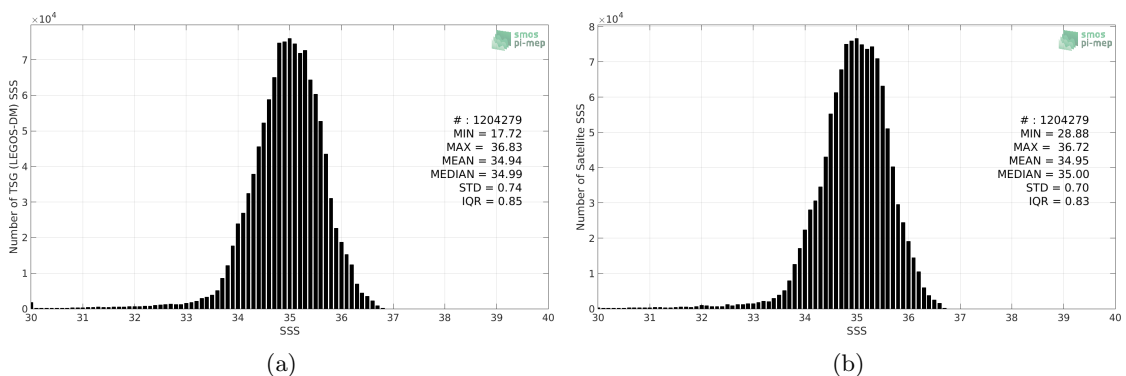
Figure 2: Histograms of SSS from TSG (LEGOS-DM) (a) and SMAP SSS L4 OI v1 - 7day (IPRC) (b) considering all match-up pairs per bins of 0.1 over the Pacific Ocean Pi-MEP region and for the full satellite product period.
