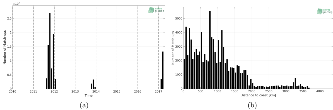
Figure 1: Number of match-ups between TSG (GOSUD-Sailing-ship) and SMAP SSS L4 OI v1 - 7 Days (IPRC) SSS as a function of time (a) and as function of the distance to coast (b) over the Pacific Ocean Pi-MEP region and for the full satellite product period.
