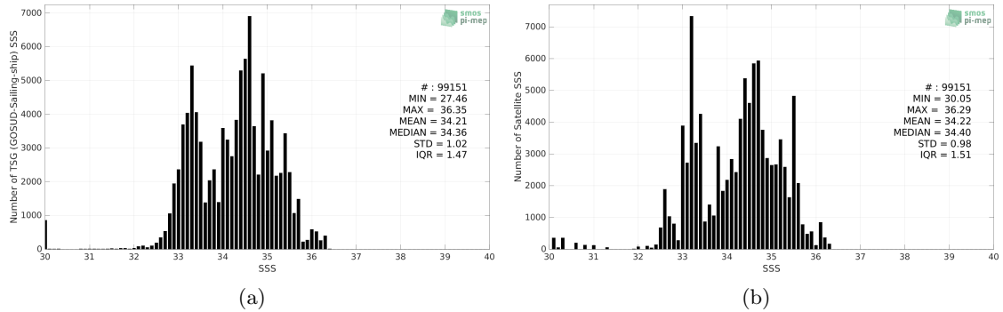
Figure 2: Histograms of SSS from TSG (GOSUD-Sailing-ship) (a) and SMAP SSS L4 OI v1 - 7 Days (IPRC) (b) considering all match-up pairs per bins of 0.1 over the Pacific Ocean Pi-MEP region and for the full satellite product period.
