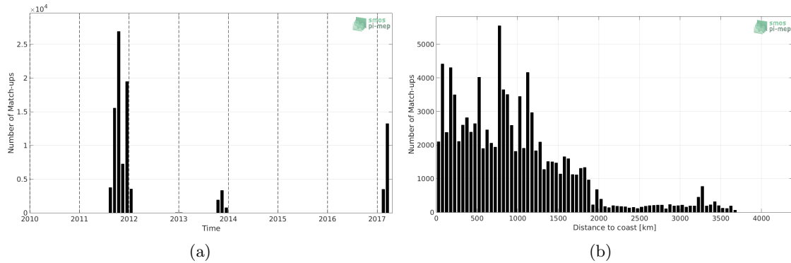
Figure 1: Number of match-ups between TSG (GOSUD-Sailing-ship) and SMAP SSS L4 OI v1 - 7day (IPRC) SSS as a function of time (a) and as function of the distance to coast (b) over the Pacific Ocean Pi-MEP region and for the full satellite product period.
