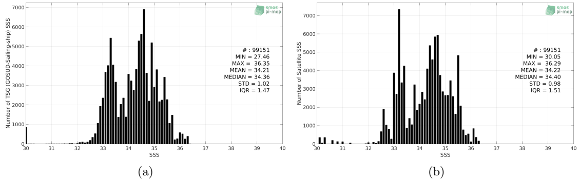
Figure 2: Histograms of SSS from TSG (GOSUD-Sailing-ship) (a) and SMAP SSS L4 OI v1 - 7day (IPRC) (b) considering all match-up pairs per bins of 0.1 over the Pacific Ocean Pi-MEP region and for the full satellite product period.
