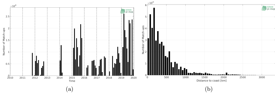
Figure 1: Number of match-ups between TSG (GOSUD-Research-vessel) and SMAP SSS L4 OI v1 - 7 Days (IPRC) SSS as a function of time (a) and as function of the distance to coast (b) over the Pacific Ocean Pi-MEP region and for the full satellite product period.
