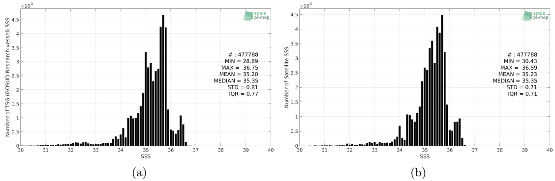
Figure 2: Histograms of SSS from TSG (GOSUD-Research-vessel) (a) and SMAP SSS L4 OI v1 - 7 Days (IPRC) (b) considering all match-up pairs per bins of 0.1 over the Pacific Ocean Pi-MEP region and for the full satellite product period.
