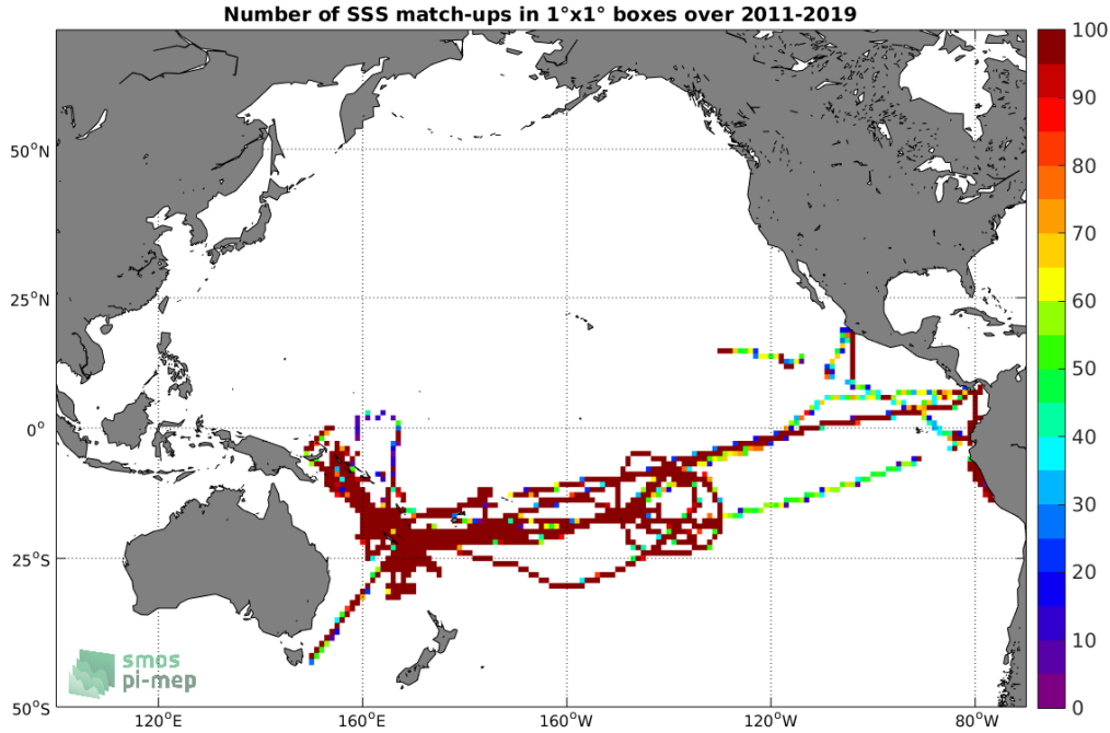
Figure 4: Number of SSS match-ups between TSG (GOSUD-Research-vessel) SSS and the SMAP SSS L4 OI v1 - 7 Days (IPRC) SSS product for the Pacific Ocean Pi-MEP region over 1^\circ \times 1^\circ boxes and for the full satellite product period.
