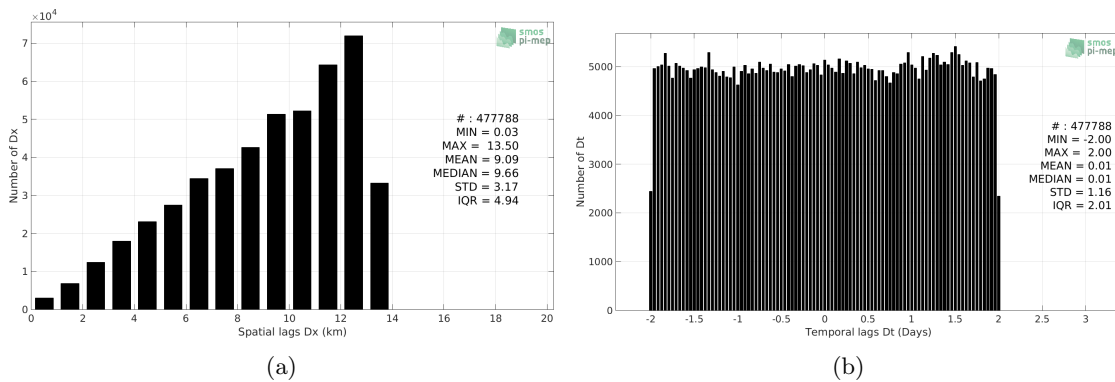
Figure 5: Histograms of the spatial (a) and temporal (b) lags between the location/time of the TSG (GOSUD-Research-vessel) measurement and the date of the corresponding SMAP SSS L4 OI v1 - 7day (IPRC) SSS pixel.
