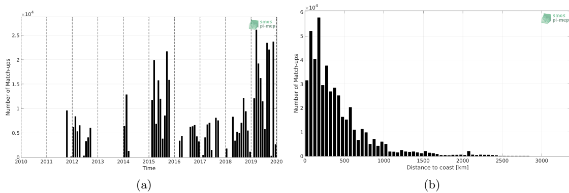
Figure 1: Number of match-ups between TSG (GOSUD-Research-vessel) and SMAP SSS L4 OI v1 - 7day (IPRC) SSS as a function of time (a) and as function of the distance to coast (b) over the Pacific Ocean Pi-MEP region and for the full satellite product period.
