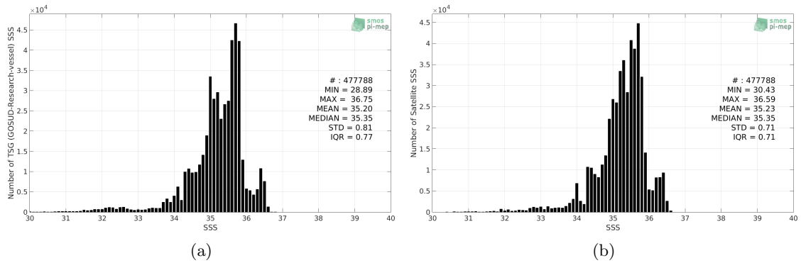
Figure 2: Histograms of SSS from TSG (GOSUD-Research-vessel) (a) and SMAP SSS L4 OI v1 - 7day (IPRC) (b) considering all match-up pairs per bins of 0.1 over the Pacific Ocean Pi-MEP region and for the full satellite product period.
