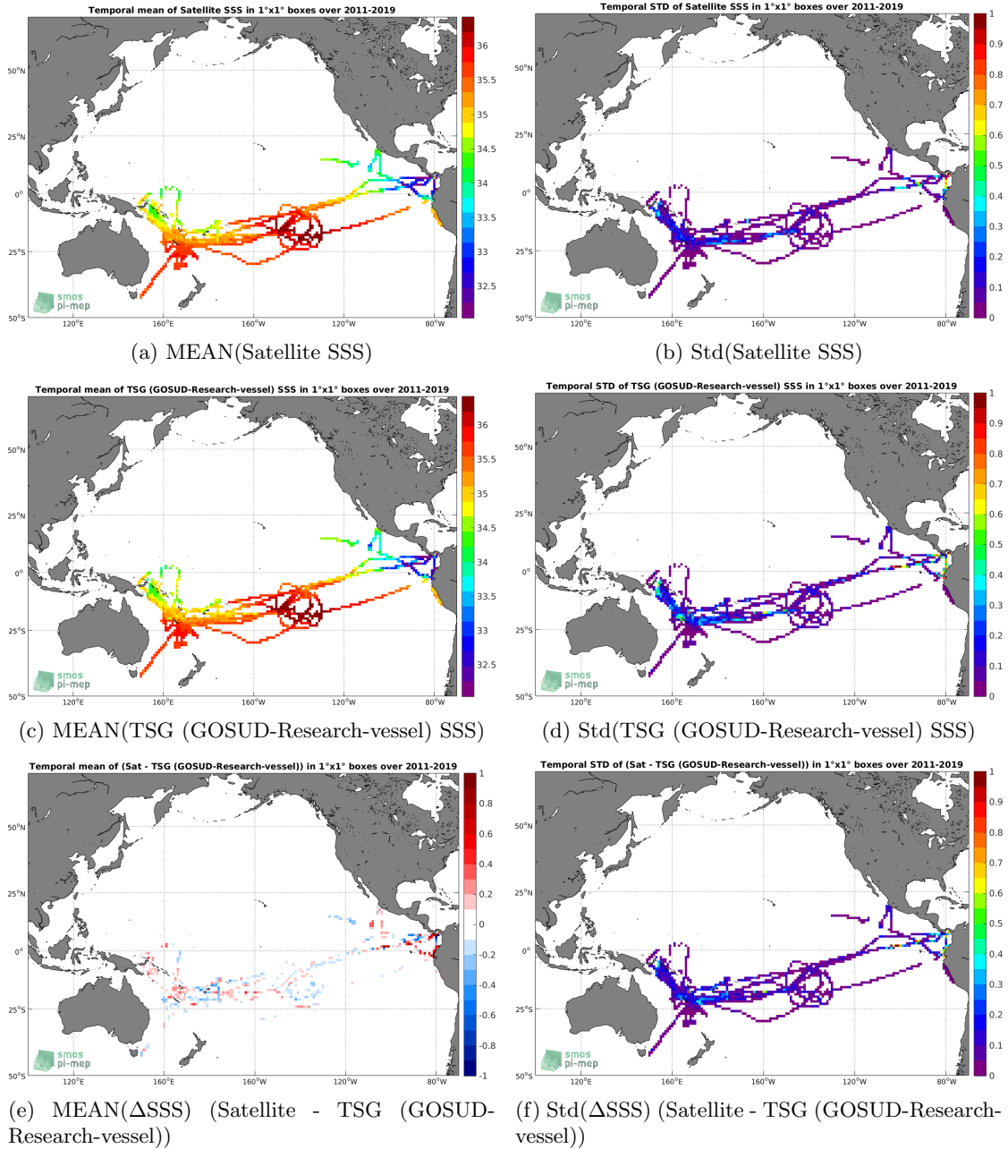
Figure 6: Temporal mean (left) and Std (right) of SSS from SMAP SSS L4 OI v1 - 7day (IPRC) (top), TSG (GOSUD-Research-vessel) (middle), and of \Delta SSS (Satellite - TSG (GOSUD-Research-vessel)). Only match-up pairs are used to generate these maps.
