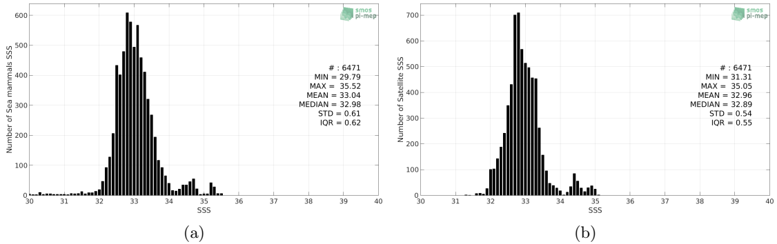
Figure 2: Histograms of SSS from Sea mammals (a) and SMAP SSS L4 OI v1 - 7day (IPRC) (b) considering all match-up pairs per bins of 0.1 over the Pacific Ocean Pi-MEP region and for the full satellite product period.
