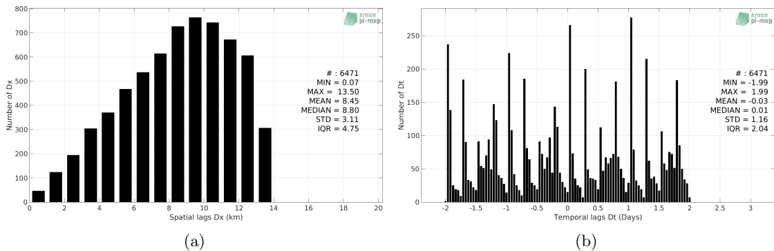
Figure 5: Histograms of the spatial (a) and temporal (b) lags between the location/time of the Sea mammals measurement and the date of the corresponding SMAP SSS L4 OI v1 - 7day (IPRC) SSS pixel.
