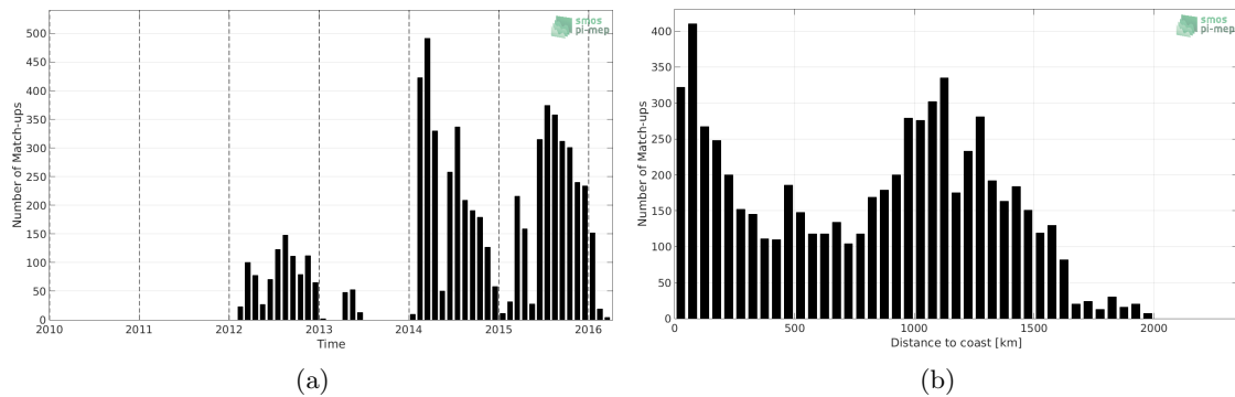
Figure 1: Number of match-ups between Sea mammals and SMAP SSS L4 OI v1 - 7day (IPRC) SSS as a function of time (a) and as function of the distance to coast (b) over the Pacific Ocean Pi-MEP region and for the full satellite product period.
