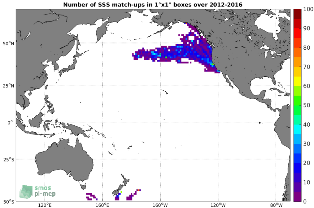
Figure 4: Number of SSS match-ups between Sea mammals SSS and the SMAP SSS L4 OI v1 - 7day (IPRC) SSS product for the Pacific Ocean Pi-MEP region over 1^\circ \times 1^\circ boxes and for the full satellite product period.
