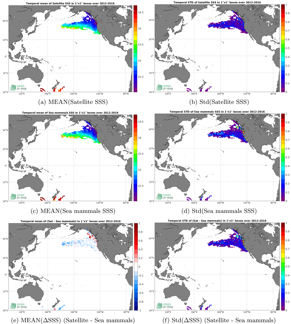
Figure 6: Temporal mean (left) and Std (right) of SSS from SMAP SSS L4 OI v1 - 7day (IPRC) (top), Sea mammals (middle), and of \Delta SSS (Satellite - Sea mammals). Only match-up pairs are used to generate these maps.
