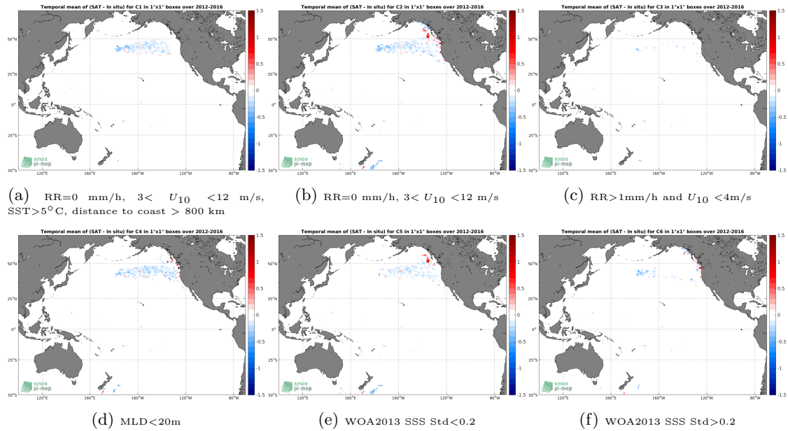
Figure 12: Temporal mean gridded over spatial boxes of size 1^\circ \times 1^\circ of \Delta SSS (SMAP SSS L4 OI v1 - 7day (IPRC) - Sea mammals) for 6 different subdatasets corresponding to:RR=0 mm/h, 3 < U_{10} < 12 m/s, SST > 5^\circ\text{C} , distance to coast > 800 km (a), RR=0 mm/h, 3 < U_{10} < 12 m/s (b), RR > 1 mm/h and U_{10} < 4 m/s (c),MLD < 20 m (d),WOA2013 SSS Std < 0.2 (e),WOA2013 SSS Std > 0.2 (f).
