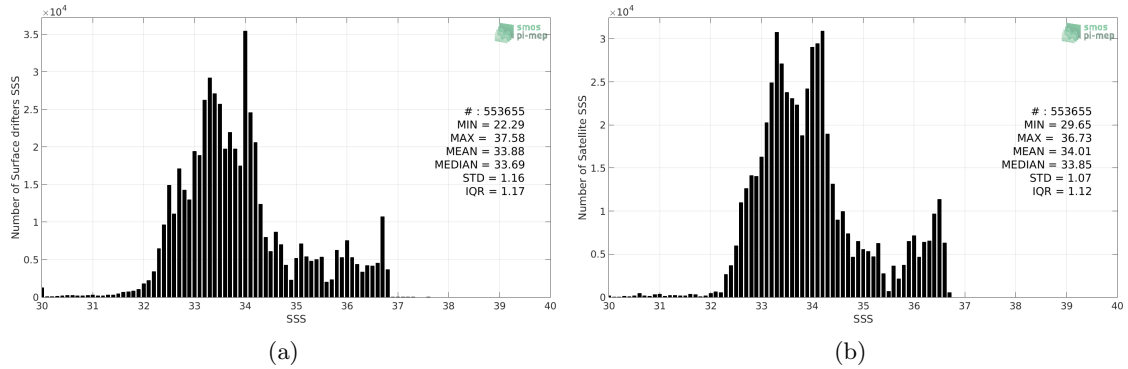
Figure 2: Histograms of SSS from Surface drifters (a) and SMAP SSS L4 OI v1 - 7day (IPRC) (b) considering all match-up pairs per bins of 0.1 over the Pacific Ocean Pi-MEP region and for the full satellite product period.
