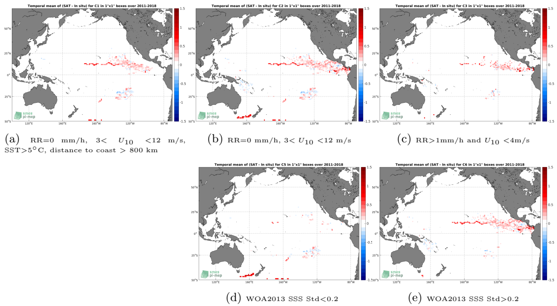
Figure 11: Temporal mean gridded over spatial boxes of size 1°x1° of \Delta SSS (SMAP SSS L4 OI v1 - 7day (IPRC) - Surface drifters) for 5 different subdatasets corresponding to:RR=0 mm/h, 3 < U_{10} < 12 m/s, SST>5°C, distance to coast > 800 km (a), RR=0 mm/h, 3 < U_{10} < 12 m/s (b), RR>1mm/h and U_{10} < 4 m/s (c), WOA2013 SSS Std<0.2 (d), WOA2013 SSS Std>0.2 (e).
