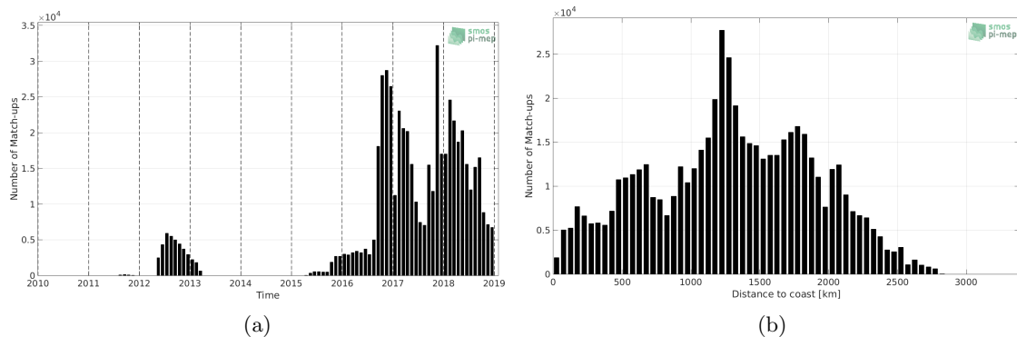
Figure 1: Number of match-ups between Surface drifters and SMAP SSS L4 OI v1 - 7day (IPRC) SSS as a function of time (a) and as function of the distance to coast (b) over the Pacific Ocean Pi-MEP region and for the full satellite product period.
