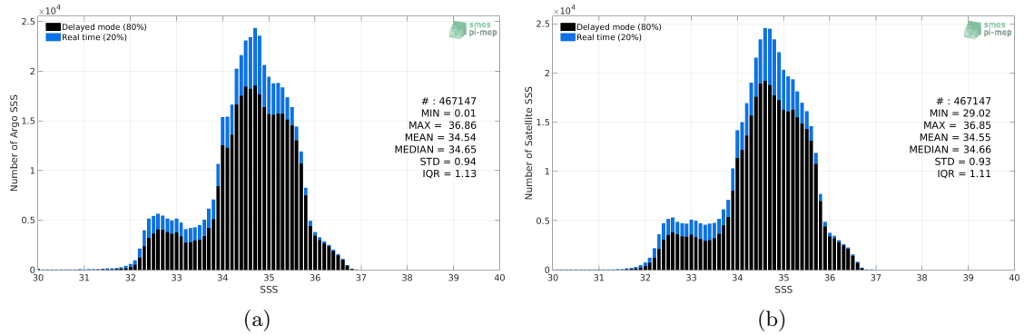
Figure 2: Histograms of SSS from Argo (a) and SMAP SSS L4 OI v1 - 7day (IPRC) (b) considering all match-up pairs per bins of 0.1 over the Pacific Ocean Pi-MEP region and for the full satellite product period.
