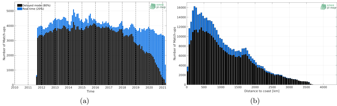
Figure 1: Number of match-ups between Argo and SMAP SSS L4 OI v1 - 7day (IPRC) SSS as a function of time (a) and as function of the distance to coast (b) over the Pacific Ocean Pi-MEP region and for the full satellite product period.
