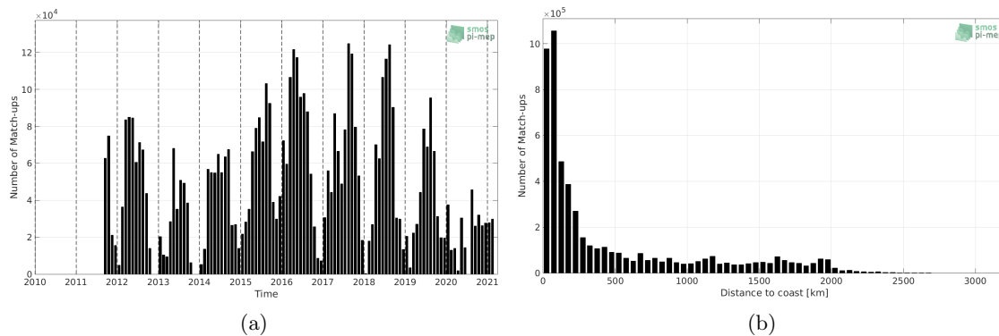
Figure 1: Number of match-ups between TSG (SAMOS) and SMAP SSS L4 OI v1 - Monthly (IPRC) SSS as a function of time (a) and as function of the distance to coast (b) over the Pacific Ocean Pi-MEP region and for the full satellite product period.
