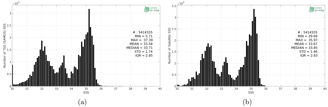
Figure 2: Histograms of SSS from TSG (SAMOS) (a) and SMAP SSS L4 OI v1 - Monthly (IPRC) (b) considering all match-up pairs per bins of 0.1 over the Pacific Ocean Pi-MEP region and for the full satellite product period.
