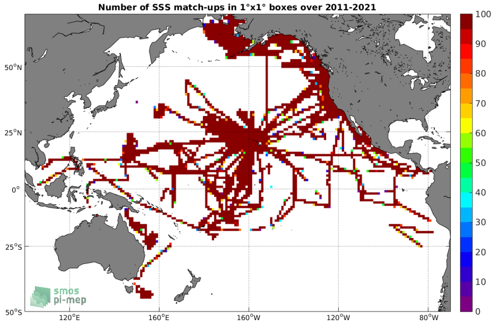
Figure 4: Number of SSS match-ups between TSG (SAMOS) SSS and the SMAP SSS L4 OI v1 - Monthly (IPRC) SSS product for the Pacific Ocean Pi-MEP region over 1^\circ \times 1^\circ boxes and for the full satellite product period.
