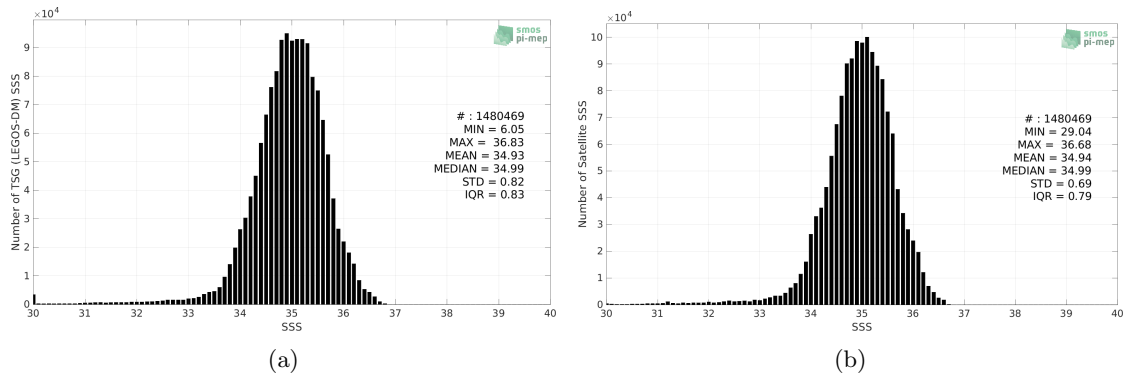
Figure 2: Histograms of SSS from TSG (LEGOS-DM) (a) and SMAP SSS L4 OI v1 - Monthly (IPRC) (b) considering all match-up pairs per bins of 0.1 over the Pacific Ocean Pi-MEP region and for the full satellite product period.
