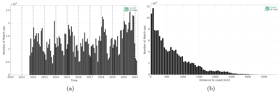
Figure 1: Number of match-ups between TSG (LEGOS-DM) and SMAP SSS L4 OI v1 - Monthly (IPRC) SSS as a function of time (a) and as function of the distance to coast (b) over the Pacific Ocean Pi-MEP region and for the full satellite product period.
