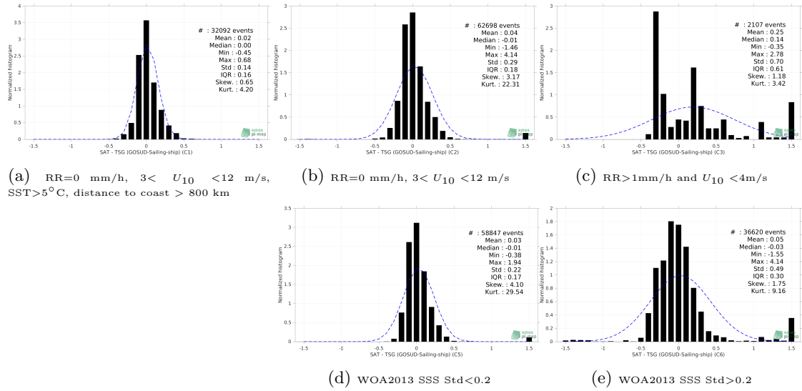
Figure 13: Normalized histogram of \Delta\text{SSS} (SMAP SSS L4 OI v1 - Monthly (IPRC) - TSG (GOSUD-Sailing-ship)) for 5 different subdatasets corresponding to: RR=0 mm/h, 3 < U_{10} < 12 m/s, SST >5^{\circ}\text{C} , distance to coast > 800 km (a), RR=0 mm/h, 3 < U_{10} < 12 m/s (b), RR >1 mm/h and U_{10} < 4 m/s (c), WOA2013 SSS Std <0.2 (d), WOA2013 SSS Std >0.2 (e).
