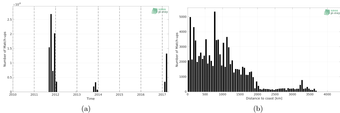
Figure 1: Number of match-ups between TSG (GOSUD-Sailing-ship) and SMAP SSS L4 OI v1 - Monthly (IPRC) SSS as a function of time (a) and as function of the distance to coast (b) over the Pacific Ocean Pi-MEP region and for the full satellite product period.
