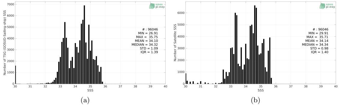
Figure 2: Histograms of SSS from TSG (GOSUD-Sailing-ship) (a) and SMAP SSS L4 OI v1 - Monthly (IPRC) (b) considering all match-up pairs per bins of 0.1 over the Pacific Ocean Pi-MEP region and for the full satellite product period.
