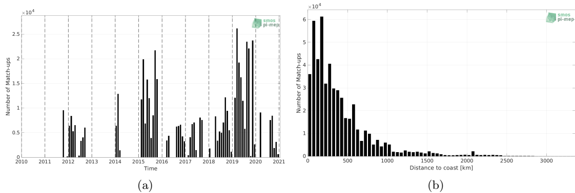
Figure 1: Number of match-ups between TSG (GOSUD-Research-vessel) and SMAP SSS L4 OI v1 - Monthly (IPRC) SSS as a function of time (a) and as function of the distance to coast (b) over the Pacific Ocean Pi-MEP region and for the full satellite product period.
