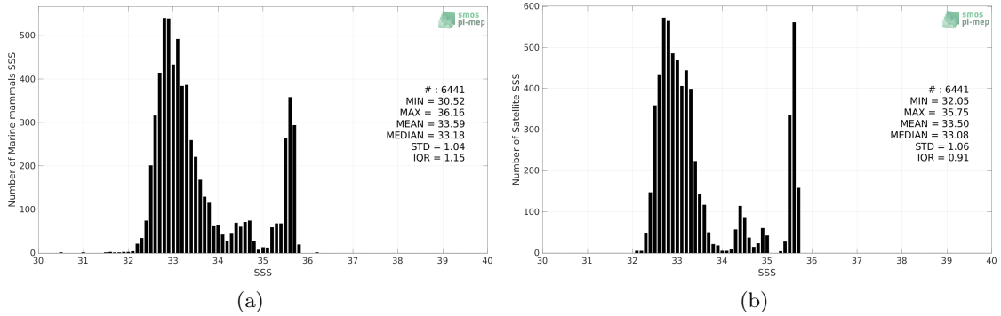
Figure 2: Histograms of SSS from Marine mammals (a) and SMAP SSS L4 OI v1 - Monthly (IPRC) (b) considering all match-up pairs per bins of 0.1 over the Pacific Ocean Pi-MEP region and for the full satellite product period.
