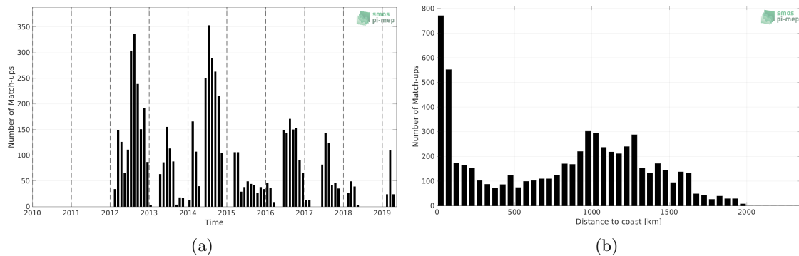
Figure 1: Number of match-ups between Marine mammals and SMAP SSS L4 OI v1 - Monthly (IPRC) SSS as a function of time (a) and as function of the distance to coast (b) over the Pacific Ocean Pi-MEP region and for the full satellite product period.
