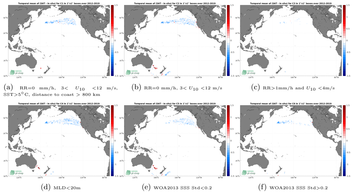
Figure 12: Temporal mean gridded over spatial boxes of size 1^\circ \times 1^\circ of \Delta SSS (SMAP SSS L4 OI v1 - Monthly (IPRC) - Marine mammals) for 6 different subdatasets corresponding to:RR=0 mm/h, 3 < U_{10} < 12 m/s, SST > 5^\circ\text{C} , distance to coast > 800 km (a), RR=0 mm/h, 3 < U_{10} < 12 m/s (b), RR > 1 mm/h and U_{10} < 4 m/s (c),MLD < 20 m (d),WOA2013 SSS Std < 0.2 (e),WOA2013 SSS Std > 0.2 (f).
