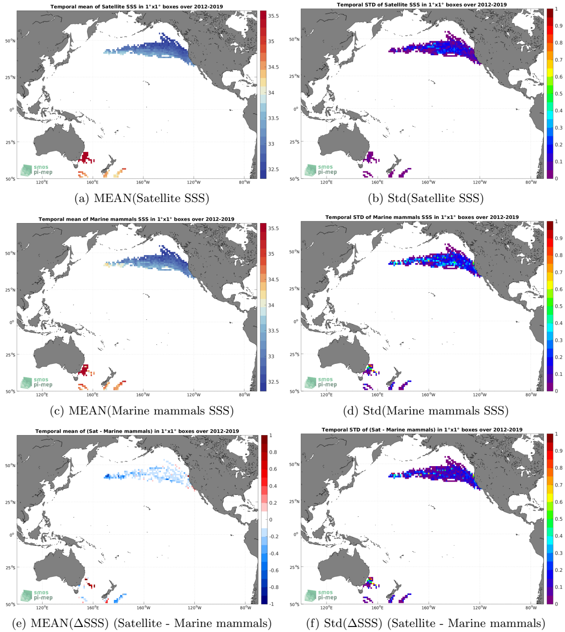
Figure 6: Temporal mean (left) and Std (right) of SSS from SMAP SSS L4 OI v1 - Monthly (IPRC) (top), Marine mammals (middle), and of \Delta SSS (Satellite - Marine mammals). Only match-up pairs are used to generate these maps.
