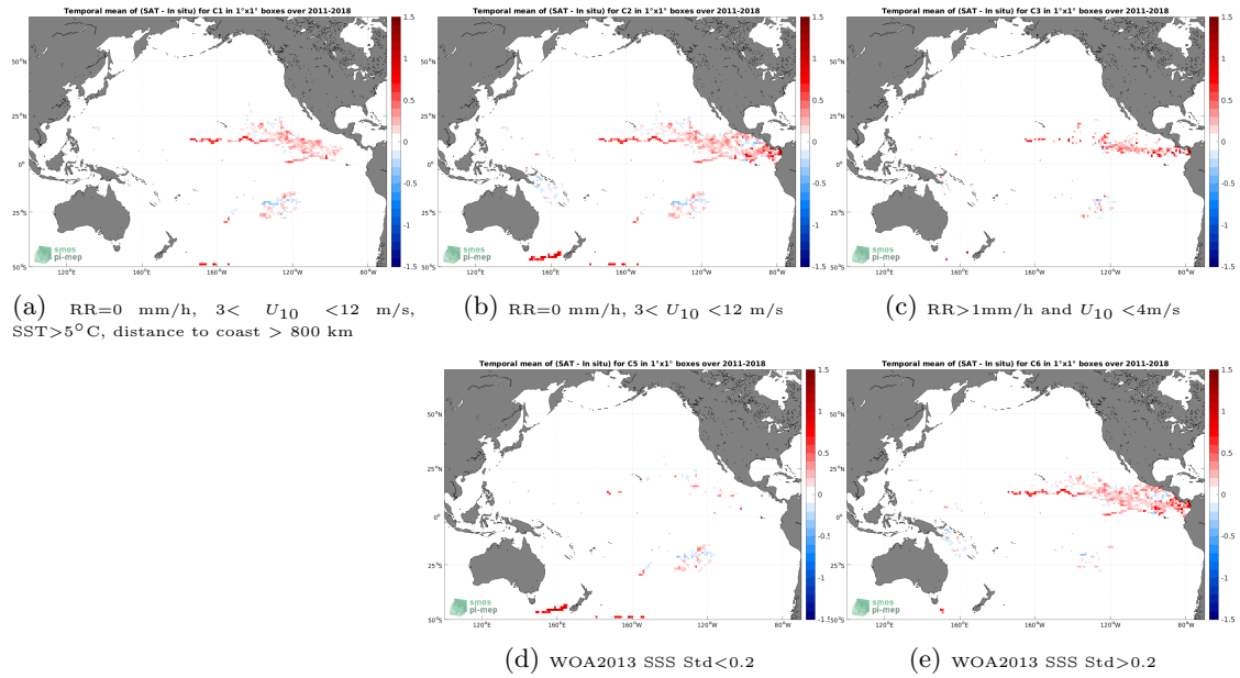
Figure 11: Temporal mean gridded over spatial boxes of size 1^\circ \times 1^\circ of \Delta SSS (SMAP SSS L4 OI v1 - Monthly (IPRC) - Surface drifters) for 5 different subdatasets corresponding to:RR=0 mm/h, 3 < U_{10} < 12 m/s, SST >5^\circ C, distance to coast > 800 km (a), RR=0 mm/h, 3 < U_{10} < 12 m/s (b), RR >1 mm/h and U_{10} < 4 m/s (c), WOA2013 SSS Std <0.2 (d), WOA2013 SSS Std >0.2 (e).
