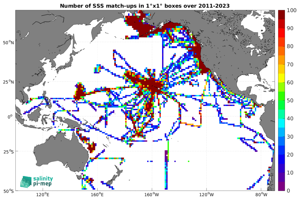
Figure 5: Number of SSS match-ups between TSG (SAMOS) SSS and the SMAP SSS L4 OI v3 - Monthly (ESR) SSS product for the Pacific Ocean Pi-MEP region over 1^\circ \times 1^\circ boxes and for the full satellite product period.
