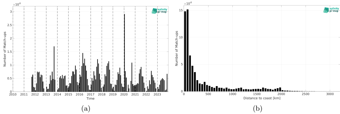
Figure 2: Number of match-ups between TSG (SAMOS) and SMAP SSS L4 OI v3 - Monthly (ESR) SSS as a function of time (a) and as function of the distance to coast (b) over the Pacific Ocean Pi-MEP region and for the full satellite product period.
