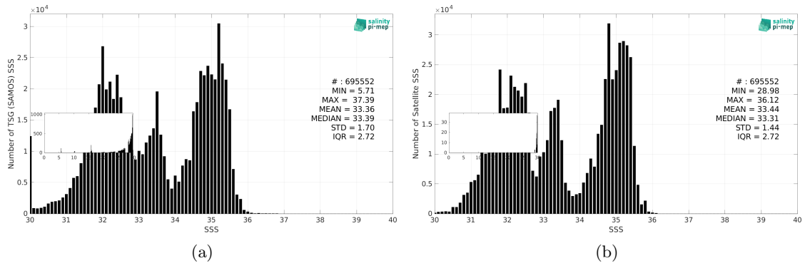
Figure 3: Histograms of SSS from TSG (SAMOS) (a) and SMAP SSS L4 OI v3 - Monthly (ESR) (b) considering all match-up pairs per bins of 0.1 over the Pacific Ocean Pi-MEP region and for the full satellite product period.
