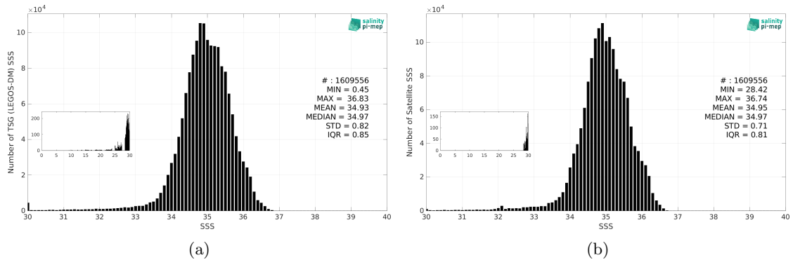
Figure 3: Histograms of SSS from TSG (LEGOS-DM) (a) and SMAP SSS L4 OI v3 - Monthly (ESR) (b) considering all match-up pairs per bins of 0.1 over the Pacific Ocean Pi-MEP region and for the full satellite product period.
