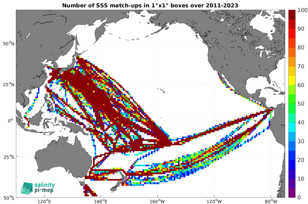
Figure 5: Number of SSS match-ups between TSG (LEGOS-DM) SSS and the SMAP SSS L4 OI v3 - Monthly (ESR) SSS product for the Pacific Ocean Pi-MEP region over 1^\circ \times 1^\circ boxes and for the full satellite product period.
