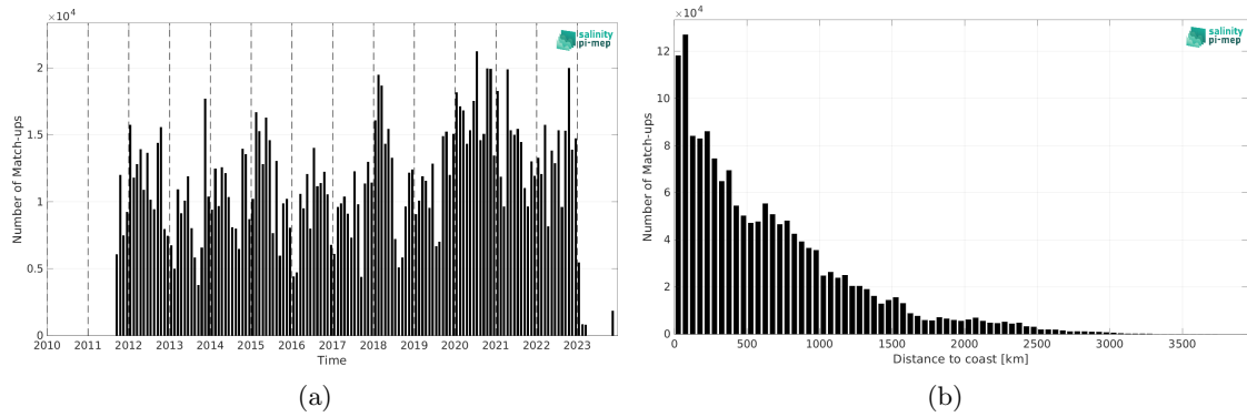
Figure 2: Number of match-ups between TSG (LEGOS-DM) and SMAP SSS L4 OI v3 - Monthly (ESR) SSS as a function of time (a) and as function of the distance to coast (b) over the Pacific Ocean Pi-MEP region and for the full satellite product period.
