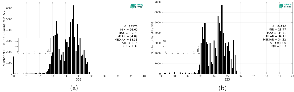
Figure 3: Histograms of SSS from TSG (GOSUD-Sailing-ship) (a) and SMAP SSS L4 OI v3 - Monthly (ESR) (b) considering all match-up pairs per bins of 0.1 over the Pacific Ocean Pi-MEP region and for the full satellite product period.
