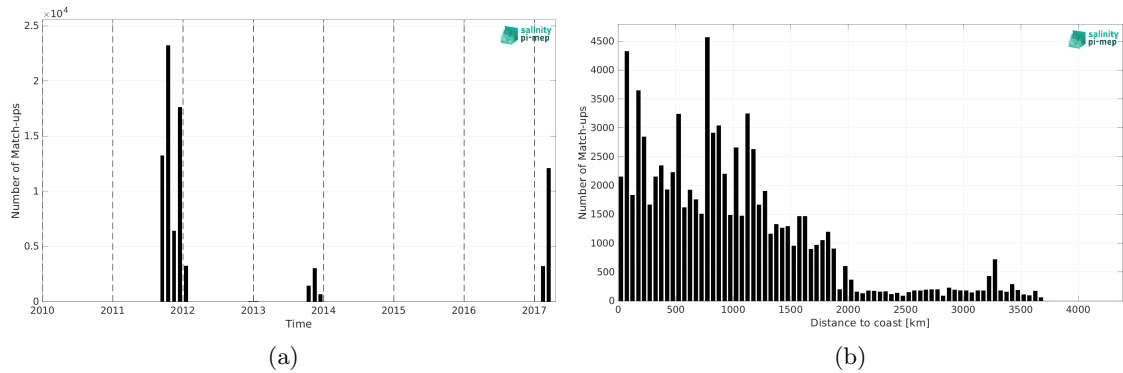
Figure 2: Number of match-ups between TSG (GOSUD-Sailing-ship) and SMAP SSS L4 OI v3 - Monthly (ESR) SSS as a function of time (a) and as function of the distance to coast (b) over the Pacific Ocean Pi-MEP region and for the full satellite product period.
