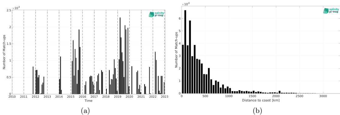
Figure 2: Number of match-ups between TSG (GOSUD-Research-vessel) and SMAP SSS L4 OI v3 - Monthly (ESR) SSS as a function of time (a) and as function of the distance to coast (b) over the Pacific Ocean Pi-MEP region and for the full satellite product period.
