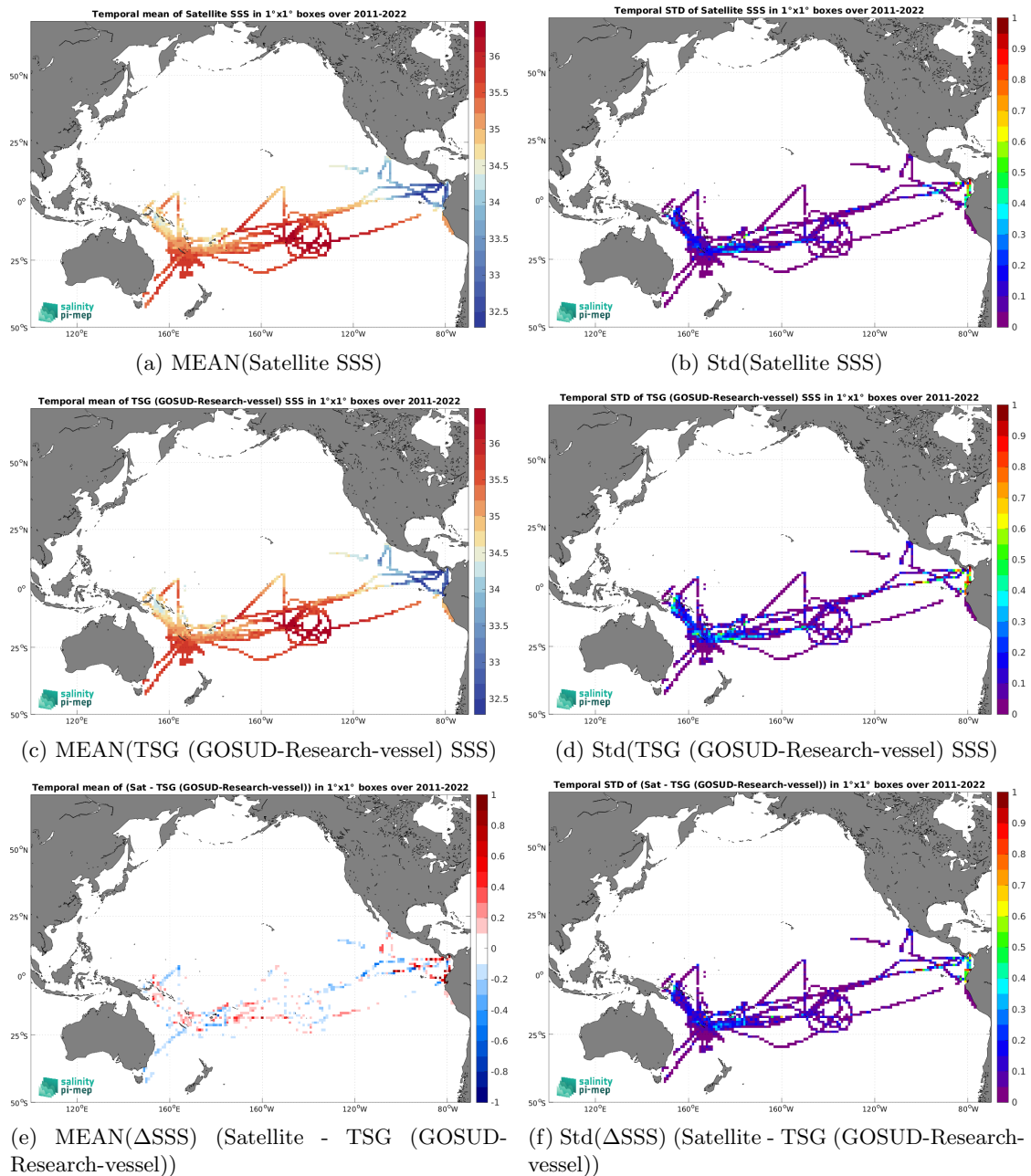
Figure 7: Temporal mean (left) and Std (right) of SSS from SMAP SSS L4 OI v3 - Monthly (ESR) (top), TSG (GOSUD-Research-vessel) (middle), and of \Delta SSS (Satellite - TSG (GOSUD-Research-vessel)). Only match-up pairs are used to generate these maps.
