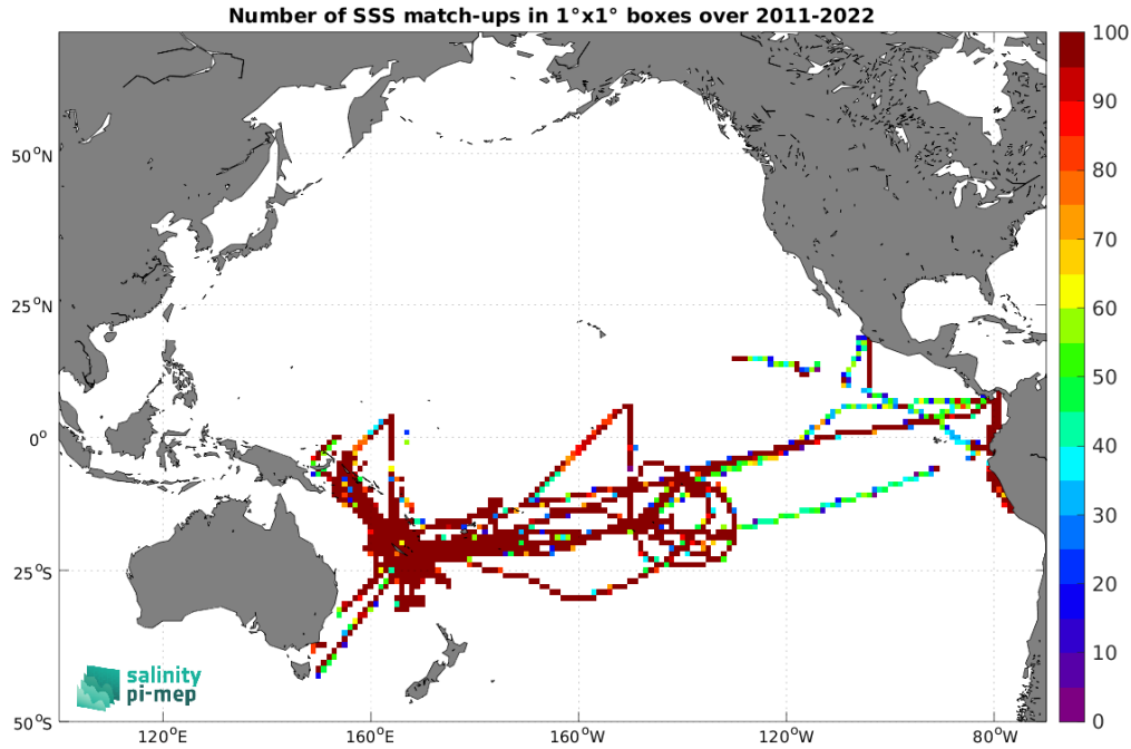
Figure 5: Number of SSS match-ups between TSG (GOSUD-Research-vessel) SSS and the SMAP SSS L4 OI v3 - Monthly (ESR) SSS product for the Pacific Ocean Pi-MEP region over 1^\circ \times 1^\circ boxes and for the full satellite product period.
