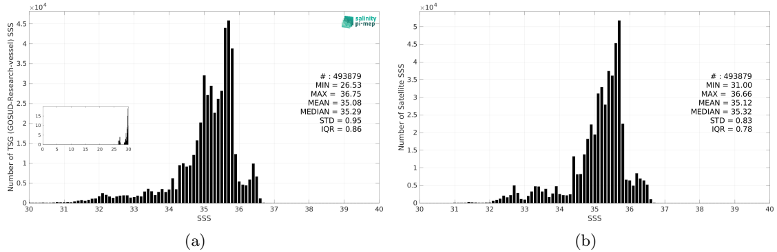
Figure 3: Histograms of SSS from TSG (GOSUD-Research-vessel) (a) and SMAP SSS L4 OI v3 - Monthly (ESR) (b) considering all match-up pairs per bins of 0.1 over the Pacific Ocean Pi-MEP region and for the full satellite product period.
