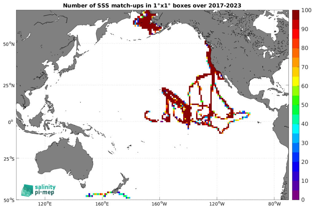
Figure 5: Number of SSS match-ups between Saildrone SSS and the SMAP SSS L4 OI v3 - Monthly (ESR) SSS product for the Pacific Ocean Pi-MEP region over 1^\circ \times 1^\circ boxes and for the full satellite product period.
