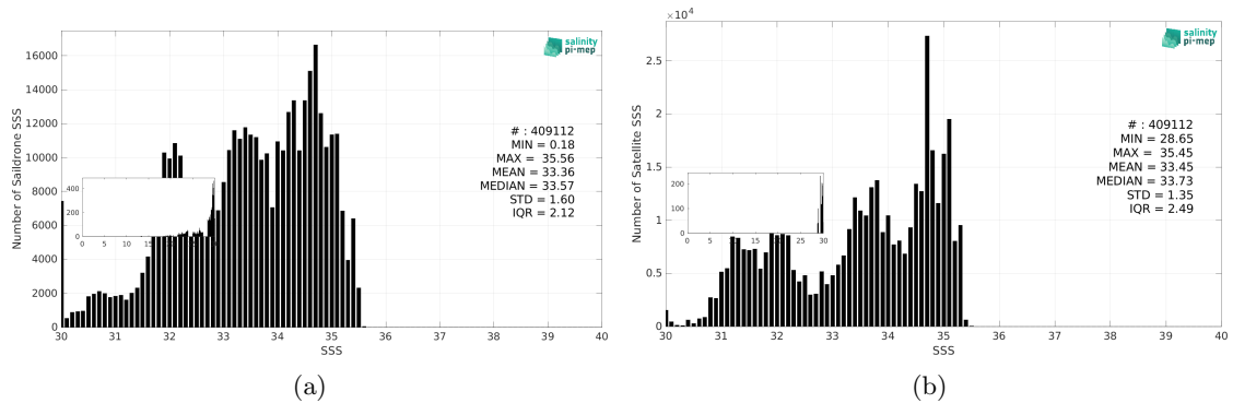
Figure 3: Histograms of SSS from Saildrone (a) and SMAP SSS L4 OI v3 - Monthly (ESR) (b) considering all match-up pairs per bins of 0.1 over the Pacific Ocean Pi-MEP region and for the full satellite product period.
