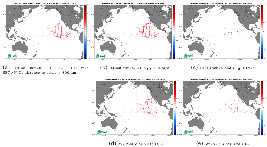
Figure 14: Temporal mean gridded over spatial boxes of size 1^\circ \times 1^\circ of \Delta SSS (SMAP SSS L4 OI v3 - Monthly (ESR) - Saildrone) for 5 different subdatasets corresponding to:RR=0 mm/h, 3 < U_{10} < 12 m/s, SST > 5^\circ\text{C} , distance to coast > 800 km (a), RR=0 mm/h, 3 < U_{10} < 12 m/s (b), RR > 1 mm/h and U_{10} < 4 m/s (c), WOA2013 SSS Std < 0.2 (d), WOA2013 SSS Std > 0.2 (e).
