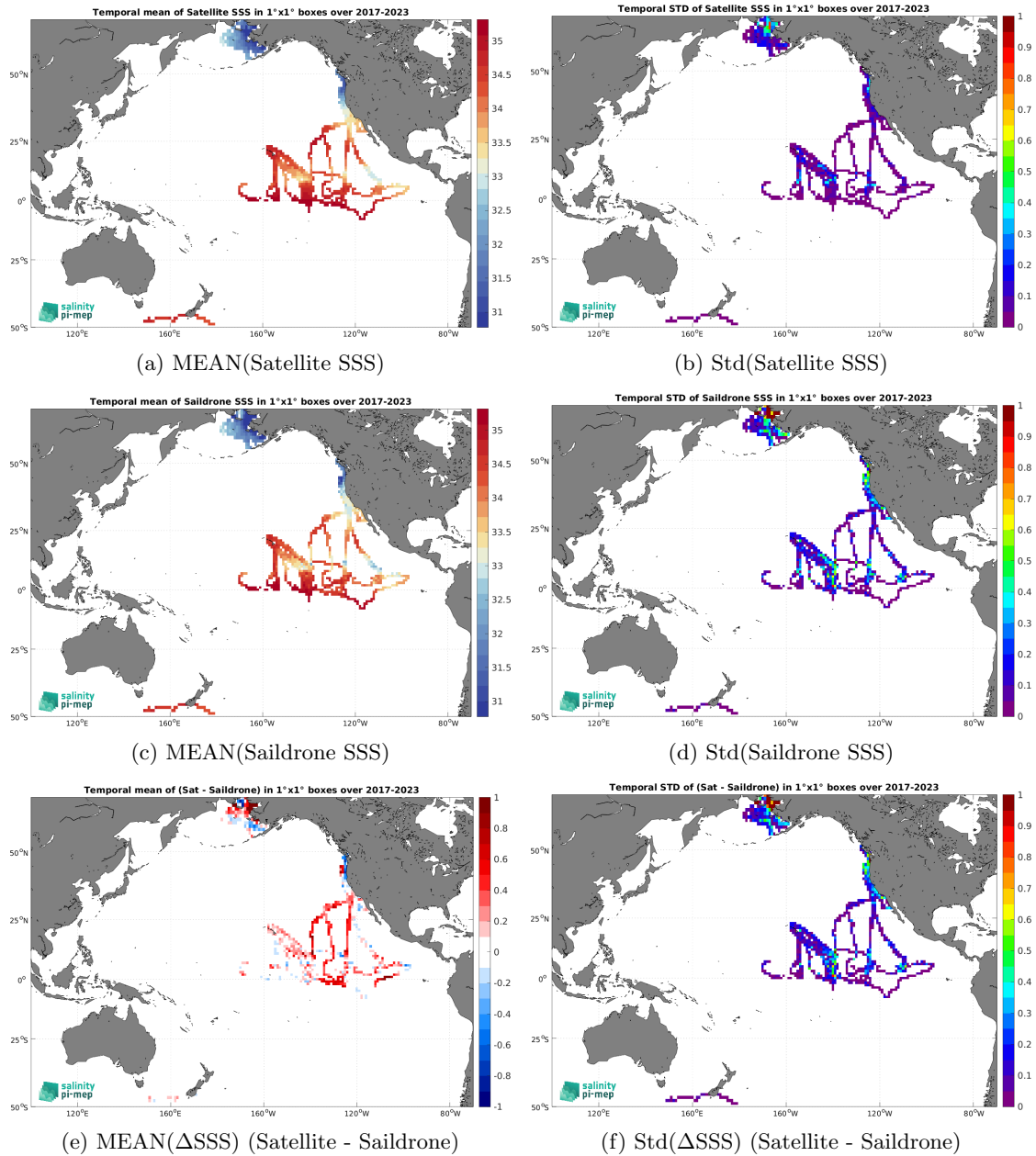
Figure 7: Temporal mean (left) and Std (right) of SSS from SMAP SSS L4 OI v3 - Monthly (ESR) (top), Saildrone (middle), and of \Delta SSS (Satellite - Saildrone). Only match-up pairs are used to generate these maps.
