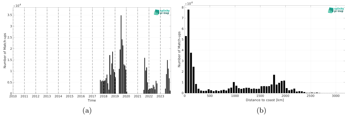
Figure 2: Number of match-ups between Saildrone and SMAP SSS L4 OI v3 - Monthly (ESR) SSS as a function of time (a) and as function of the distance to coast (b) over the Pacific Ocean Pi-MEP region and for the full satellite product period.
