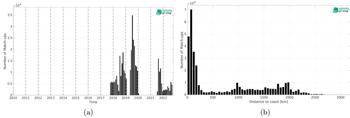
Figure 2: Number of match-ups between Sailldrone and SMAP SSS L4 OI v3 - Monthly (ESR) SSS as a function of time (a) and as function of the distance to coast (b) over the Pacific Ocean Pi-MEP region and for the full satellite product period.
