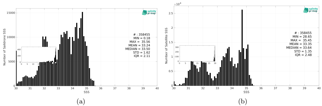
Figure 3: Histograms of SSS from Sailldrone (a) and SMAP SSS L4 OI v3 - Monthly (ESR) (b) considering all match-up pairs per bins of 0.1 over the Pacific Ocean Pi-MEP region and for the full satellite product period.
