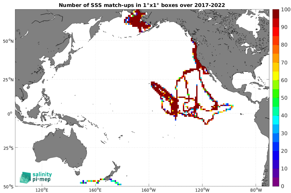
Figure 5: Number of SSS match-ups between Saildrone SSS and the SMAP SSS L4 OI v3 - Monthly (ESR) SSS product for the Pacific Ocean Pi-MEP region over 1°×1° boxes and for the full satellite product period.
