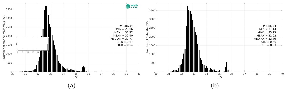
Figure 3: Histograms of SSS from Marine mammals (a) and SMAP SSS L4 OI v3 - Monthly (ESR) (b) considering all match-up pairs per bins of 0.1 over the Pacific Ocean Pi-MEP region and for the full satellite product period.
