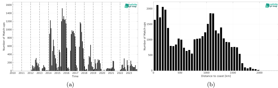
Figure 2: Number of match-ups between Marine mammals and SMAP SSS L4 OI v3 - Monthly (ESR) SSS as a function of time (a) and as function of the distance to coast (b) over the Pacific Ocean Pi-MEP region and for the full satellite product period.
