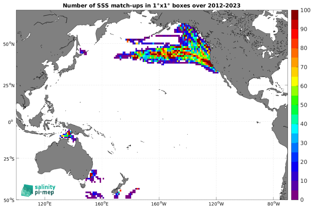
Figure 5: Number of SSS match-ups between Marine mammals SSS and the SMAP SSS L4 OI v3 - Monthly (ESR) SSS product for the Pacific Ocean Pi-MEP region over 1^\circ \times 1^\circ boxes and for the full satellite product period.
