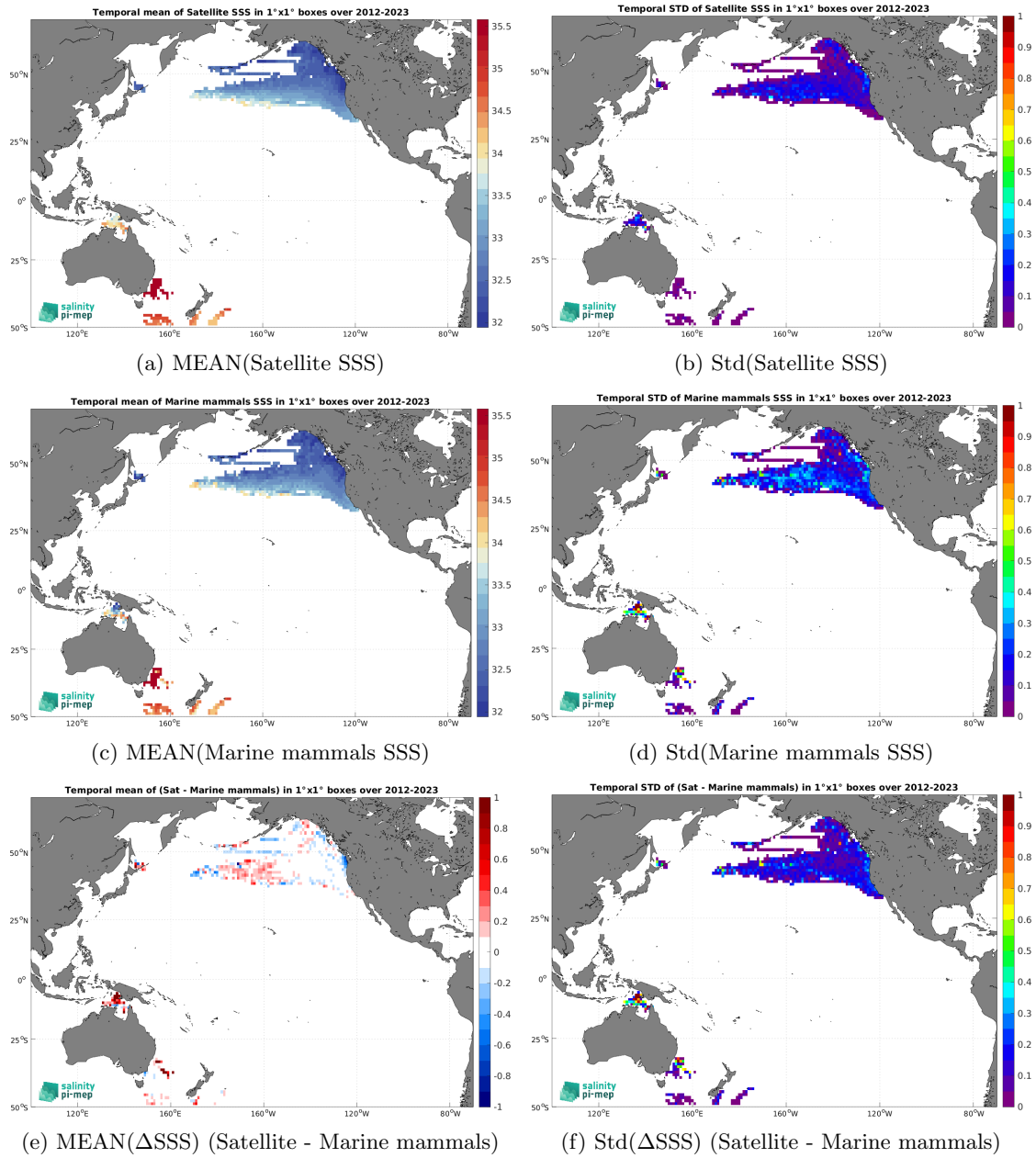
Figure 7: Temporal mean (left) and Std (right) of SSS from SMAP SSS L4 OI v3 - Monthly (ESR) (top), Marine mammals (middle), and of \Delta SSS (Satellite - Marine mammals). Only match-up pairs are used to generate these maps.
