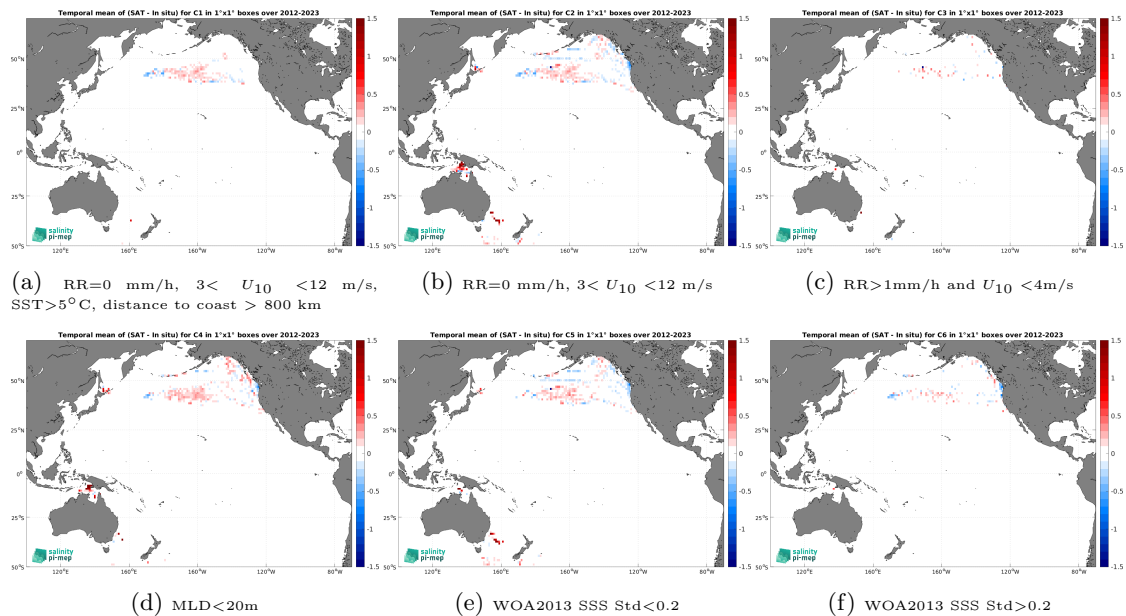
Figure 14: Temporal mean gridded over spatial boxes of size 1^\circ \times 1^\circ of \Delta SSS (SMAP SSS L4 OI v3 - Monthly (ESR) - Marine mammals) for 6 different subdatasets corresponding to:RR=0 mm/h, 3 < U_{10} < 12 m/s, SST >5^\circ C, distance to coast > 800 km (a), RR=0 mm/h, 3 < U_{10} < 12 m/s (b), RR >1 mm/h and U_{10} < 4 m/s (c),MLD <20 m (d),WOA2013 SSS Std <0.2 (e),WOA2013 SSS Std >0.2 (f).
