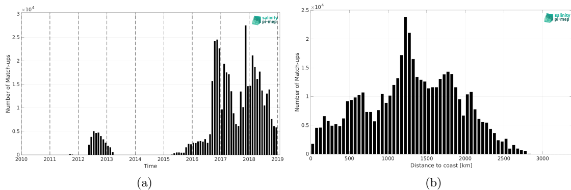
Figure 2: Number of match-ups between Surface drifters and SMAP SSS L4 OI v3 - Monthly (ESR) SSS as a function of time (a) and as function of the distance to coast (b) over the Pacific Ocean Pi-MEP region and for the full satellite product period.
