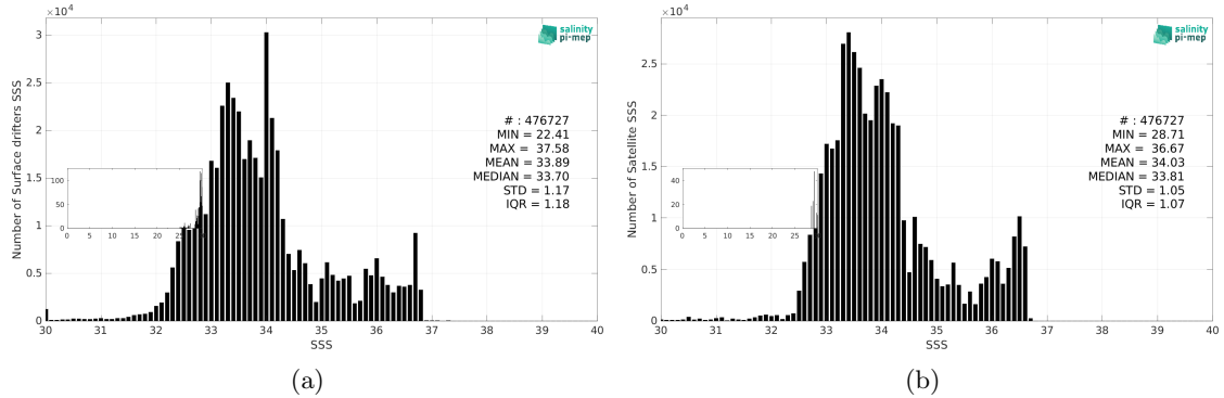
Figure 3: Histograms of SSS from Surface drifters (a) and SMAP SSS L4 OI v3 - Monthly (ESR) (b) considering all match-up pairs per bins of 0.1 over the Pacific Ocean Pi-MEP region and for the full satellite product period.
