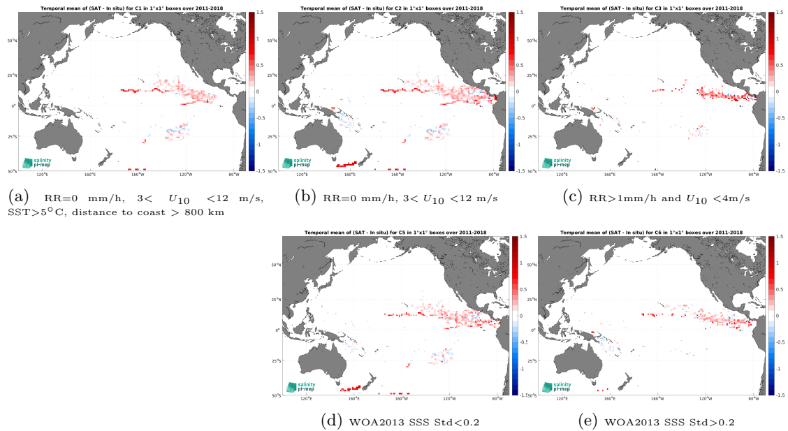
Figure 13: Temporal mean gridded over spatial boxes of size 1^\circ \times 1^\circ of \Delta SSS (SMAP SSS L4 OI v3 - Monthly (ESR) - Surface drifters) for 5 different subdatasets corresponding to:RR=0 mm/h, 3 < U_{10} < 12 m/s, SST >5^\circ C, distance to coast > 800 km (a), RR=0 mm/h, 3 < U_{10} < 12 m/s (b), RR >1 mm/h and U_{10} < 4 m/s (c), WOA2013 SSS Std <0.2 (d), WOA2013 SSS Std >0.2 (e).
