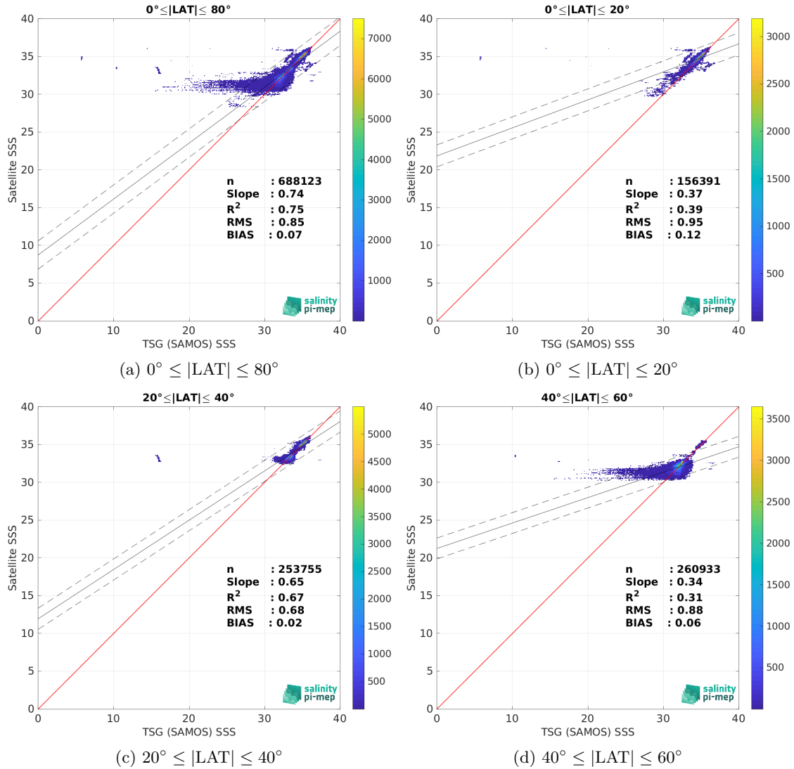
Figure 10: Contour maps of the concentration of SMAP SSS L4 OI v3 - Daily (ESR) SSS (y-axis) versus TSG (SAMOS) SSS (x-axis) at match-up pairs for different latitude bands. For each plot, the red line shows x=y . The black thin and dashed lines indicate a linear fit through the data cloud and the \pm 95\% confidence levels, respectively. The number match-up pairs n , the slope and R^2 coefficient of the linear fit, the root mean square (RMS) and the mean bias between satellite and in situ data are indicated for each latitude band in each plots.
