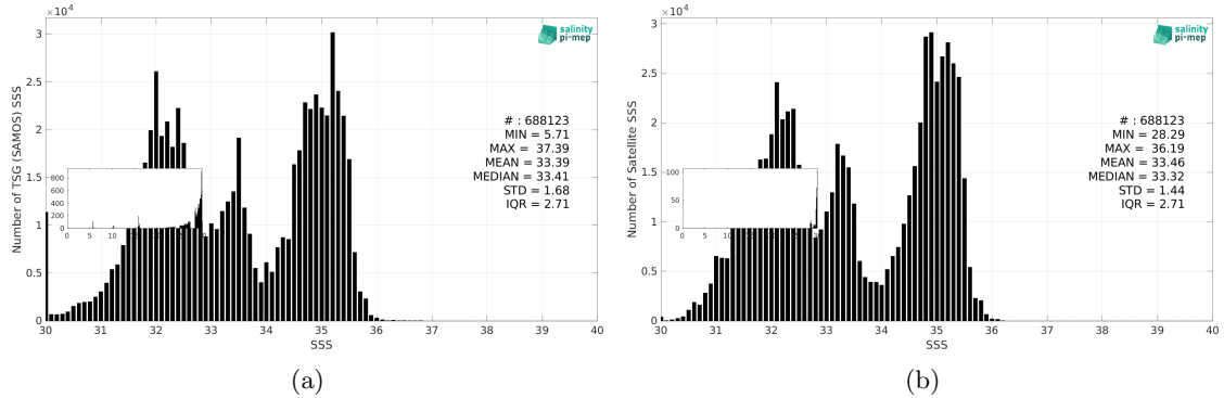
Figure 3: Histograms of SSS from TSG (SAMOS) (a) and SMAP SSS L4 OI v3 - Daily (ESR) (b) considering all match-up pairs per bins of 0.1 over the Pacific Ocean Pi-MEP region and for the full satellite product period.
