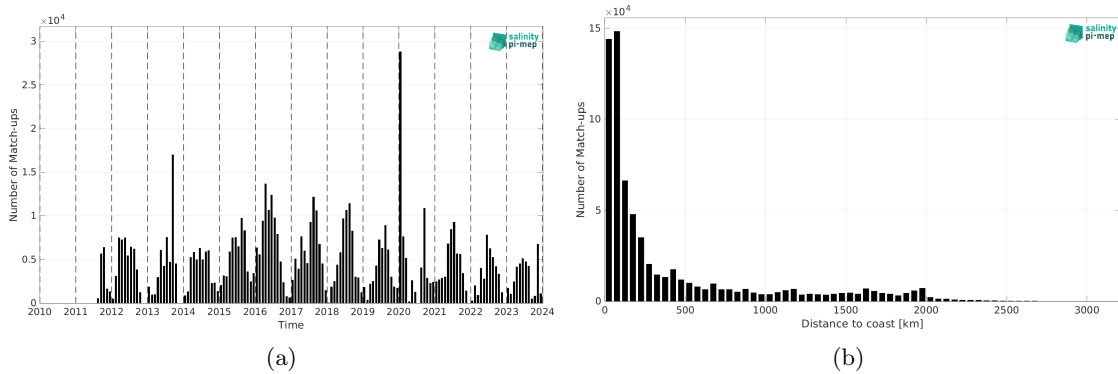
Figure 2: Number of match-ups between TSG (SAMOS) and SMAP SSS L4 OI v3 - Daily (ESR) SSS as a function of time (a) and as function of the distance to coast (b) over the Pacific Ocean Pi-MEP region and for the full satellite product period.
