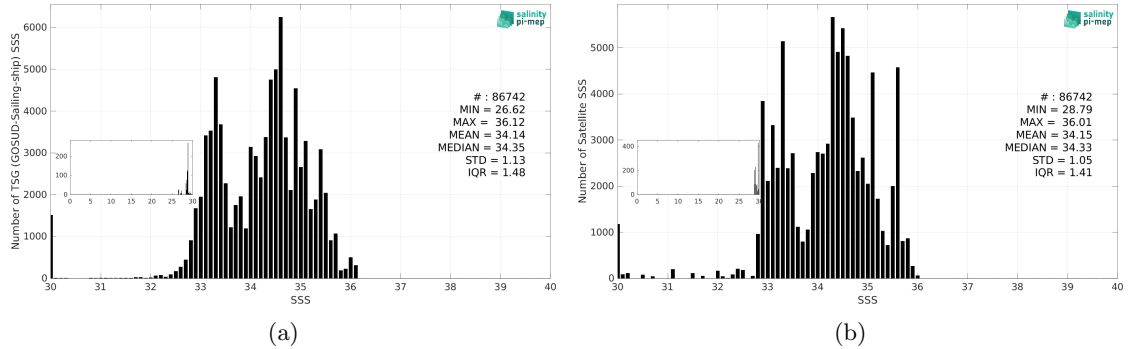
Figure 3: Histograms of SSS from TSG (GOSUD-Sailing-ship) (a) and SMAP SSS L4 OI v3 - Daily (ESR) (b) considering all match-up pairs per bins of 0.1 over the Pacific Ocean Pi-MEP region and for the full satellite product period.
