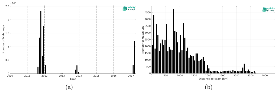
Figure 2: Number of match-ups between TSG (GOSUD-Sailing-ship) and SMAP SSS L4 OI v3 - Daily (ESR) SSS as a function of time (a) and as function of the distance to coast (b) over the Pacific Ocean Pi-MEP region and for the full satellite product period.
