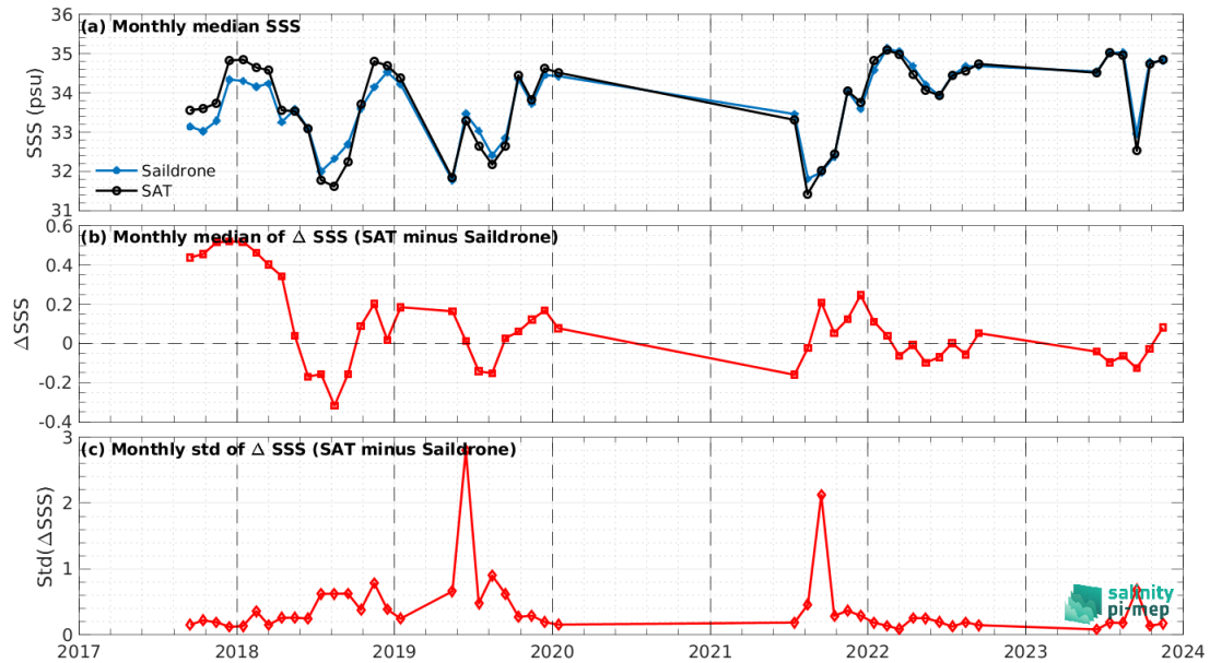
Figure 8: Time series of the monthly median SSS (top), median of \Delta\text{SSS} (Satellite - Sairdronne) and Std of \Delta\text{SSS} (Satellite - Sairdronne) over the Pacific Ocean Pi-MEP region considering all match-ups collected by the Pi-MEP.
