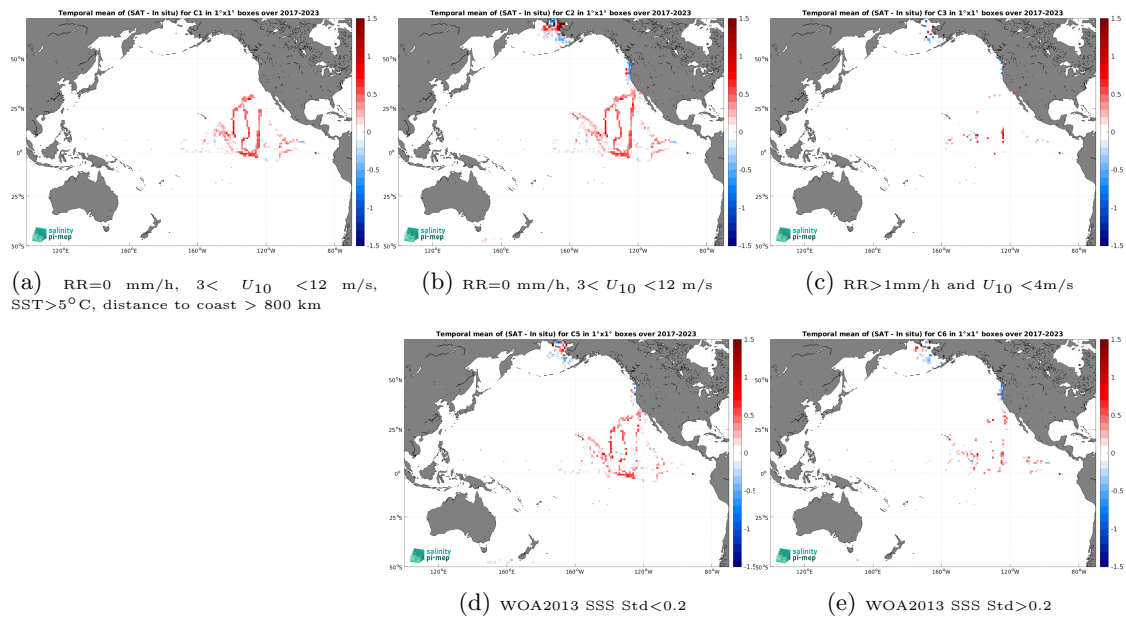
Figure 14: Temporal mean gridded over spatial boxes of size 1^\circ \times 1^\circ of \Delta SSS (SMAP SSS L4 OI v3 - Daily (ESR) - Saildrone) for 5 different subdatasets corresponding to: RR=0 mm/h, 3 < U_{10} < 12 m/s, SST > 5^\circ\text{C} , distance to coast > 800 km (a), RR=0 mm/h, 3 < U_{10} < 12 m/s (b), RR > 1 mm/h and U_{10} < 4 m/s (c), WOA2013 SSS Std < 0.2 (d), WOA2013 SSS Std > 0.2 (e).
