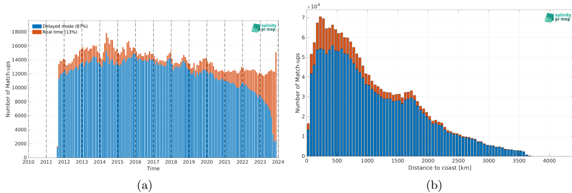
Figure 2: Number of match-ups between Argo and SMAP SSS L4 OI v3 - Daily (ESR) SSS as a function of time (a) and as function of the distance to coast (b) over the Pacific Ocean Pi-MEP region and for the full satellite product period.
