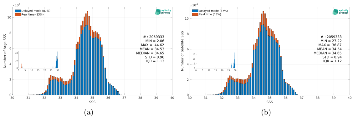
Figure 3: Histograms of SSS from Argo (a) and SMAP SSS L4 OI v3 - Daily (ESR) (b) considering all match-up pairs per bins of 0.1 over the Pacific Ocean Pi-MEP region and for the full satellite product period.
