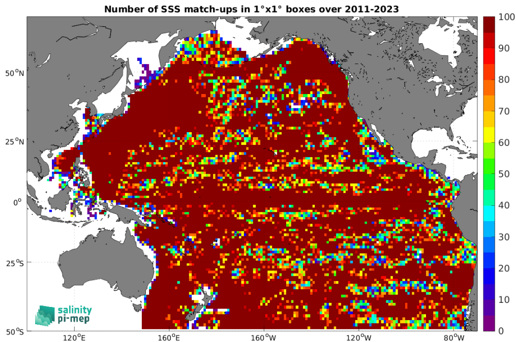
Figure 5: Number of SSS match-ups between Argo SSS and the SMAP SSS L4 OI v3 - Daily (ESR) SSS product for the Pacific Ocean Pi-MEP region over 1^\circ \times 1^\circ boxes and for the full satellite product period.
