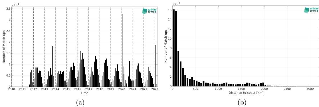
Figure 1: Number of match-ups between TSG (SAMOS) and SMAP SSS L4 OI v2 - 7 Days (ESR) SSS as a function of time (a) and as function of the distance to coast (b) over the Pacific Ocean Pi-MEP region and for the full satellite product period.
