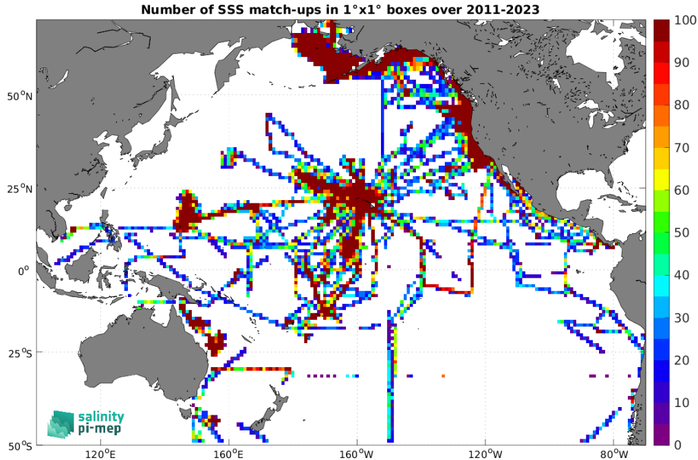
Figure 4: Number of SSS match-ups between TSG (SAMOS) SSS and the SMAP SSS L4 OI v2 - 7 Days (ESR) SSS product for the Pacific Ocean Pi-MEP region over 1^\circ \times 1^\circ boxes and for the full satellite product period.
