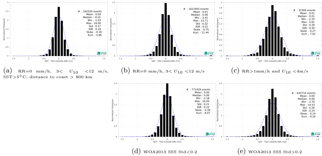
Figure 13: Normalized histogram of \Delta\text{SSS} (SMAP SSS L4 OI v2 - 7 Days (ESR) - TSG (LEGOS-DM)) for 5 different subdatasets corresponding to: RR=0 mm/h, 3 < U_{10} < 12 m/s, SST>5°C, distance to coast > 800 km (a), RR=0 mm/h, 3 < U_{10} < 12 m/s (b), RR>1mm/h and U_{10} < 4 m/s (c), WOA2013 SSS Std<0.2 (d), WOA2013 SSS Std>0.2 (e).
