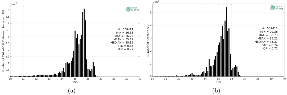
Figure 2: Histograms of SSS from TSG (GOSUD-Research-vessel) (a) and SMAP SSS L4 OI v2 - 7 Days (ESR) (b) considering all match-up pairs per bins of 0.1 over the Pacific Ocean Pi-MEP region and for the full satellite product period.
