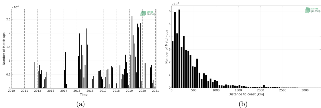
Figure 1: Number of match-ups between TSG (GOSUD-Research-vessel) and SMAP SSS L4 OI v2 - 7 Days (ESR) SSS as a function of time (a) and as function of the distance to coast (b) over the Pacific Ocean Pi-MEP region and for the full satellite product period.
