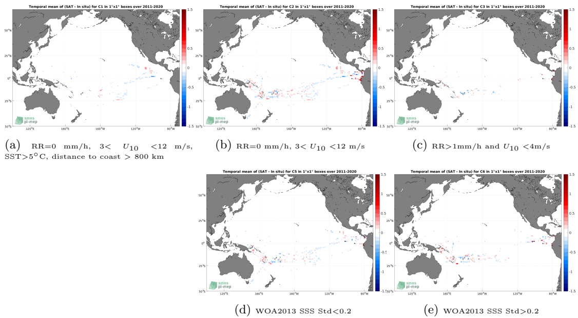
Figure 12: Temporal mean gridded over spatial boxes of size 1^\circ \times 1^\circ of \Delta SSS (SMAP SSS L4 OI v2 - 7 Days (ESR) - TSG (GOSUD-Research-vessel)) for 5 different subdatasets corresponding to:RR=0 mm/h, 3 < U_{10} < 12 m/s, SST>5°C, distance to coast > 800 km (a), RR=0 mm/h, 3 < U_{10} < 12 m/s (b), RR>1mm/h and U_{10} < 4 m/s (c), WOA2013 SSS Std<0.2 (d), WOA2013 SSS Std>0.2 (e).
