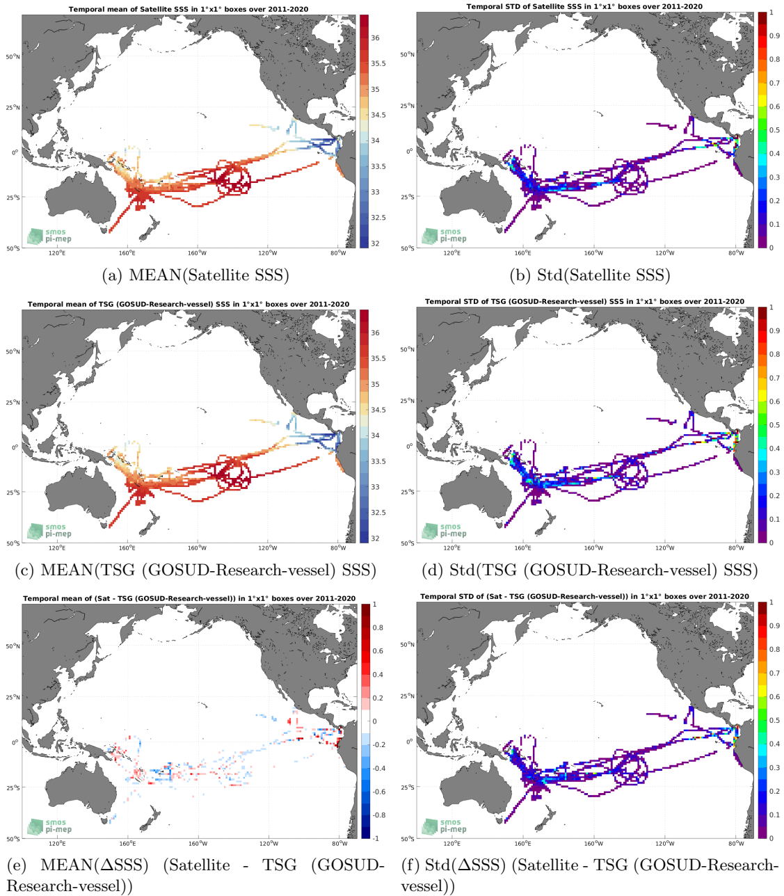
Figure 6: Temporal mean (left) and Std (right) of SSS from SMAP SSS L4 OI v2 - 7 Days (ESR) (top), TSG (GOSUD-Research-vessel) (middle), and of \Delta SSS (Satellite - TSG (GOSUD-Research-vessel)). Only match-up pairs are used to generate these maps.
