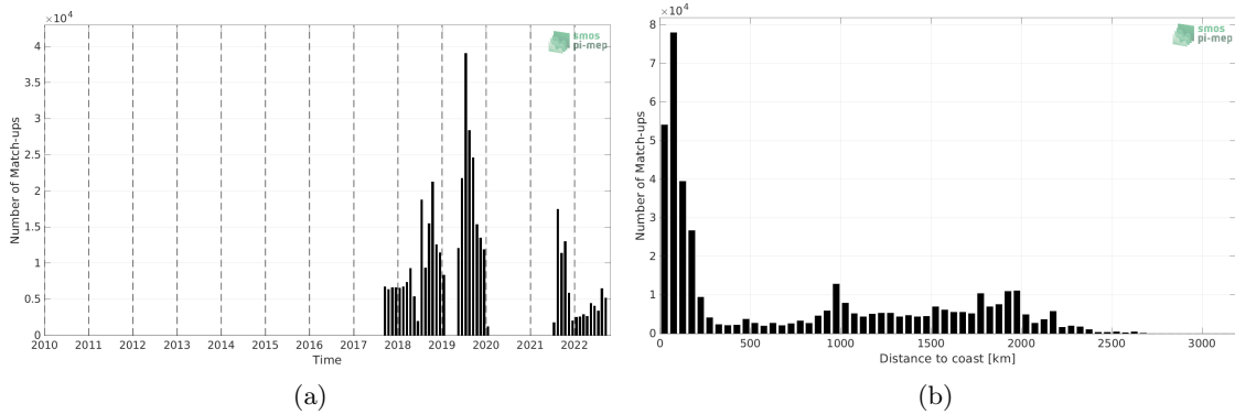
Figure 1: Number of match-ups between Saildrone and SMAP SSS L4 OI v2 - 7 Days (ESR) SSS as a function of time (a) and as function of the distance to coast (b) over the Pacific Ocean Pi-MEP region and for the full satellite product period.
