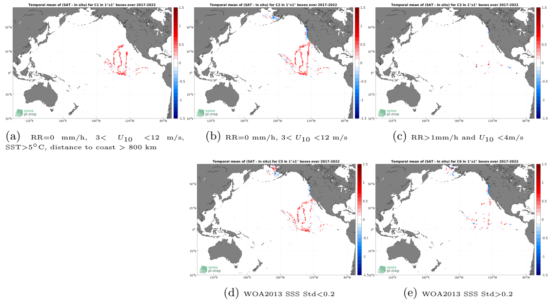
Figure 12: Temporal mean gridded over spatial boxes of size 1^\circ \times 1^\circ of \Delta SSS (SMAP SSS L4 OI v2 - 7 Days (ESR) - Sairdrone) for 5 different subdatasets corresponding to:RR=0 mm/h, 3 < U_{10} < 12 m/s, SST >5^\circ C, distance to coast > 800 km (a), RR=0 mm/h, 3 < U_{10} < 12 m/s (b), RR >1 mm/h and U_{10} < 4 m/s (c), WOA2013 SSS Std <0.2 (d), WOA2013 SSS Std >0.2 (e).
