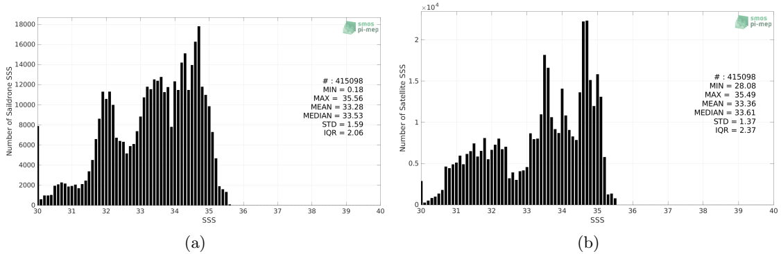
Figure 2: Histograms of SSS from Saildrone (a) and SMAP SSS L4 OI v2 - 7 Days (ESR) (b) considering all match-up pairs per bins of 0.1 over the Pacific Ocean Pi-MEP region and for the full satellite product period.
