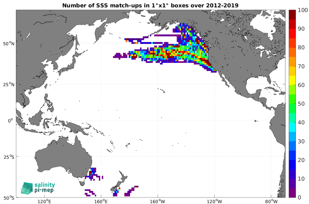
Figure 4: Number of SSS match-ups between Marine mammals SSS and the SMAP SSS L4 OI v2 - 7 Days (ESR) SSS product for the Pacific Ocean Pi-MEP region over 1^\circ \times 1^\circ boxes and for the full satellite product period.
