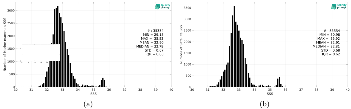
Figure 2: Histograms of SSS from Marine mammals (a) and SMAP SSS L4 OI v2 - 7 Days (ESR) (b) considering all match-up pairs per bins of 0.1 over the Pacific Ocean Pi-MEP region and for the full satellite product period.
