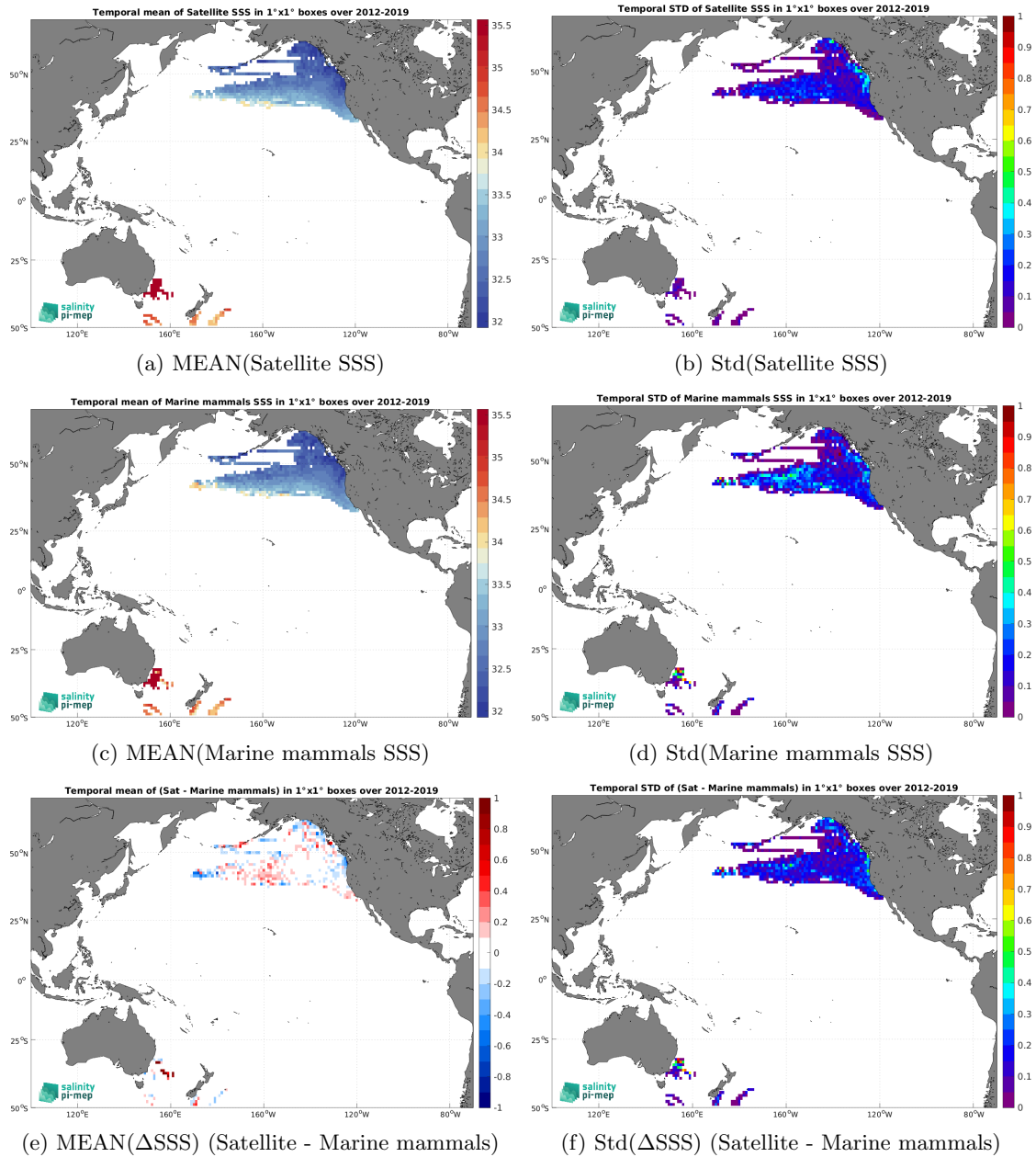
Figure 6: Temporal mean (left) and Std (right) of SSS from SMAP SSS L4 OI v2 - 7 Days (ESR) (top), Marine mammals (middle), and of \Delta SSS (Satellite - Marine mammals). Only match-up pairs are used to generate these maps.
