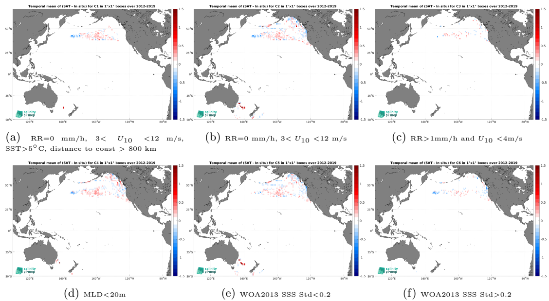
Figure 12: Temporal mean gridded over spatial boxes of size 1^\circ \times 1^\circ of \Delta SSS (SMAP SSS L4 OI v2 - 7 Days (ESR) - Marine mammals) for 6 different subdatasets corresponding to:RR=0 mm/h, 3 < U_{10} < 12 m/s, SST > 5^\circ C, distance to coast > 800 km (a), RR=0 mm/h, 3 < U_{10} < 12 m/s (b), RR > 1 mm/h and U_{10} < 4 m/s (c),MLD < 20 m (d),WOA2013 SSS Std < 0.2 (e),WOA2013 SSS Std > 0.2 (f).
