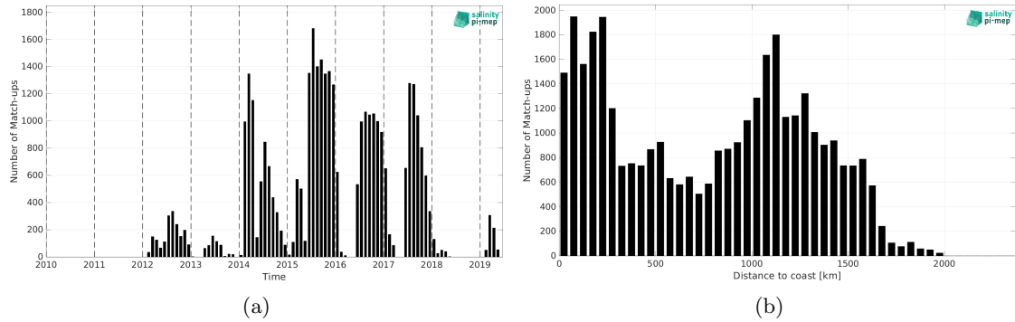
Figure 1: Number of match-ups between Marine mammals and SMAP SSS L4 OI v2 - 7 Days (ESR) SSS as a function of time (a) and as function of the distance to coast (b) over the Pacific Ocean Pi-MEP region and for the full satellite product period.
