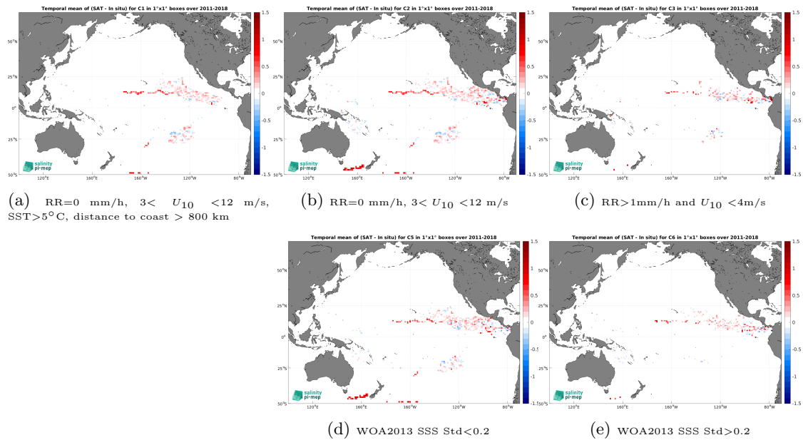
Figure 11: Temporal mean gridded over spatial boxes of size 1^\circ \times 1^\circ of \Delta SSS (SMAP SSS L4 OI v2 - 7 Days (ESR) - Surface drifters) for 5 different subdatasets corresponding to:RR=0 mm/h, 3 < U_{10} < 12 m/s, SST >5^\circ C, distance to coast > 800 km (a), RR=0 mm/h, 3 < U_{10} < 12 m/s (b), RR >1 mm/h and U_{10} < 4 m/s (c), WOA2013 SSS Std <0.2 (d), WOA2013 SSS Std >0.2 (e).
