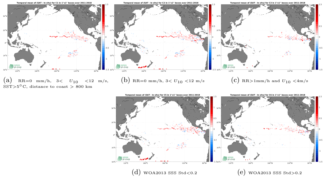
Figure 11: Temporal mean gridded over spatial boxes of size 1^\circ \times 1^\circ of \Delta SSS (SMAP SSS L4 OI v2 - 7 Days (ESR) - Surface drifters) for 5 different subdatasets corresponding to: RR=0 mm/h, 3 < U_{10} < 12 m/s, SST > 5^\circ\text{C} , distance to coast > 800 km (a), RR=0 mm/h, 3 < U_{10} < 12 m/s (b), RR > 1 mm/h and U_{10} < 4 m/s (c), WOA2013 SSS Std < 0.2 (d), WOA2013 SSS Std > 0.2 (e).
