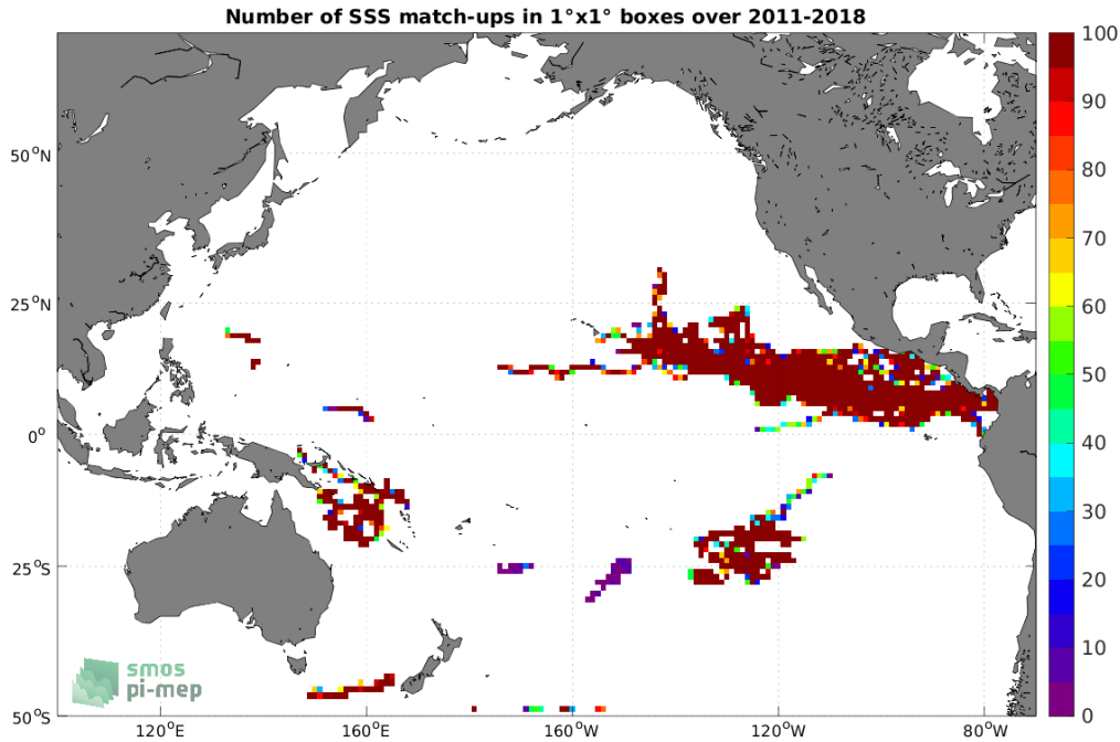
Figure 3: Number of SSS match-ups between Surface drifters SSS and the SMAP SSS L4 OI v2 - 7 Days (ESR) SSS product for the Pacific Ocean Pi-MEP region over 1^\circ \times 1^\circ boxes and for the full satellite product period.
