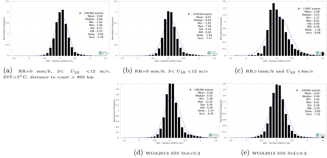
Figure 12: Normalized histogram of \Delta SSS (SMAP SSS L4 OI v2 - 7 Days (ESR) - Surface drifters) for 5 different subdatasets corresponding to: RR=0 mm/h, 3 < U_{10} < 12 m/s, SST > 5°C, distance to coast > 800 km (a), RR=0 mm/h, 3 < U_{10} < 12 m/s (b), RR > 1mm/h and U_{10} < 4 m/s (c), WOA2013 SSS Std < 0.2 (d), WOA2013 SSS Std > 0.2 (e).
