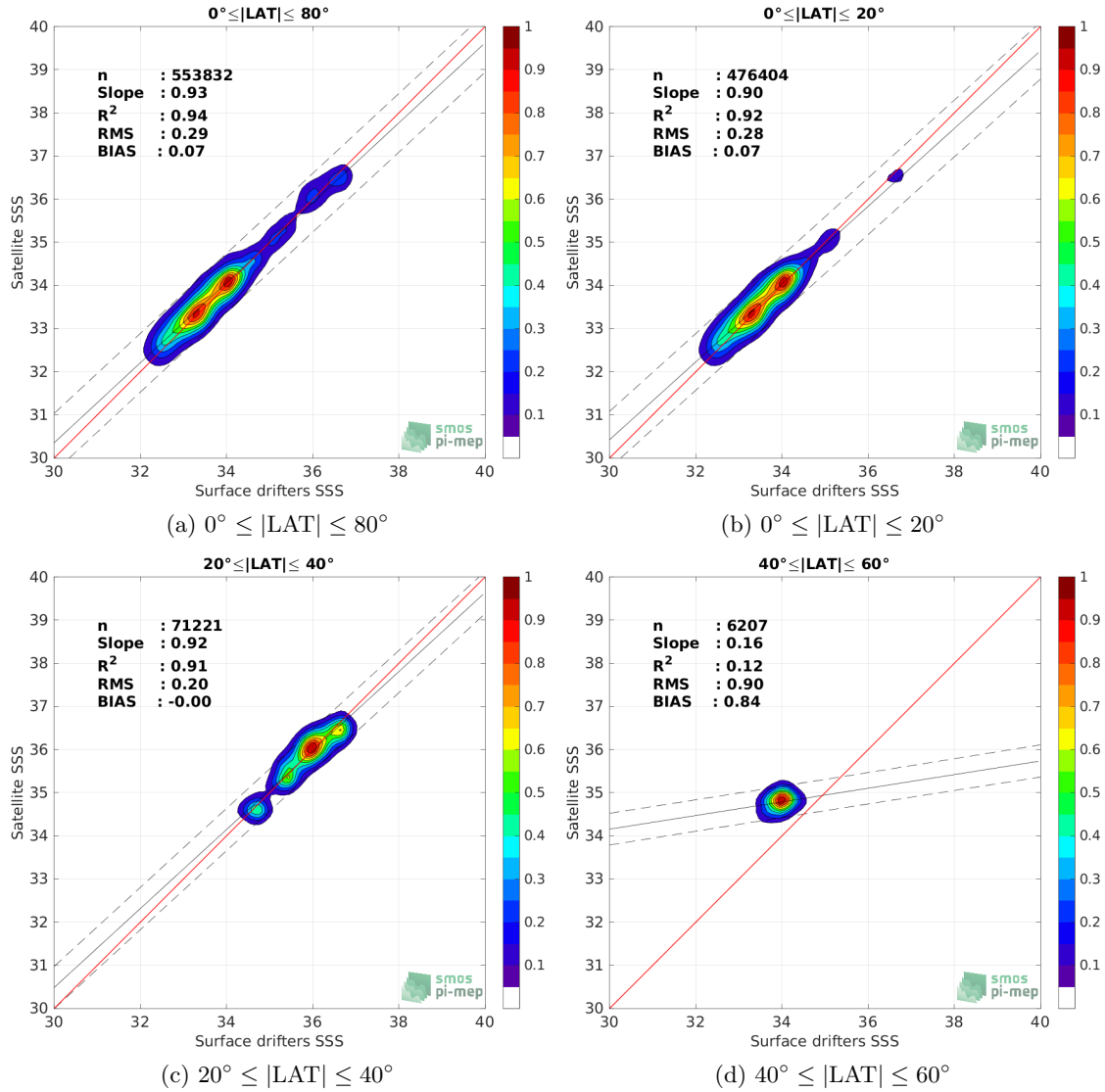
Figure 8: Contour maps of the concentration of SMAP SSS L4 OI v2 - 7 Days (ESR) SSS (y-axis) versus Surface drifters SSS (x-axis) at match-up pairs for different latitude bands. For each plot, the red line shows x=y . The black thin and dashed lines indicate a linear fit through the data cloud and the \pm 95\% confidence levels, respectively. The number match-up pairs n , the slope and R^2 coefficient of the linear fit, the root mean square (RMS) and the mean bias between satellite and in situ data are indicated for each latitude band in each plots.
