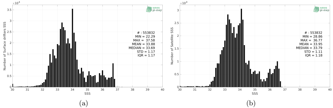
Figure 2: Histograms of SSS from Surface drifters (a) and SMAP SSS L4 OI v2 - 7 Days (ESR) (b) considering all match-up pairs per bins of 0.1 over the Pacific Ocean Pi-MEP region and for the full satellite product period.
