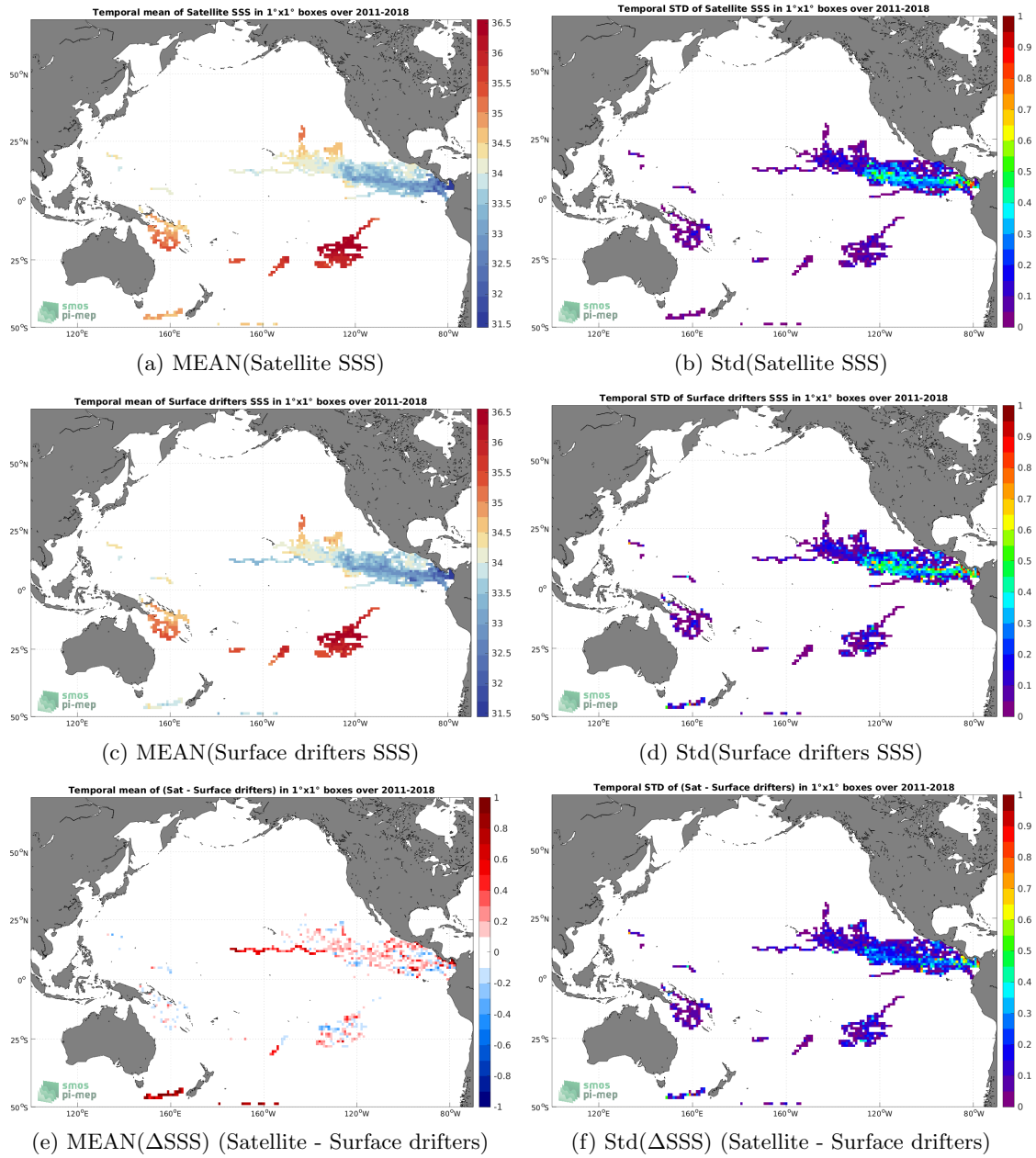
Figure 5: Temporal mean (left) and Std (right) of SSS from SMAP SSS L4 OI v2 - 7 Days (ESR) (top), Surface drifters (middle), and of \Delta SSS (Satellite - Surface drifters). Only match-up pairs are used to generate these maps.
