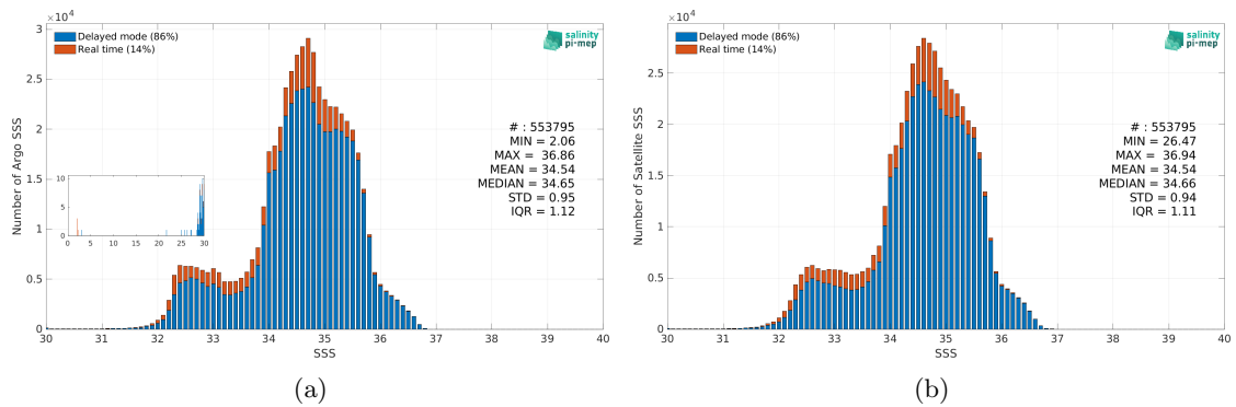
Figure 2: Histograms of SSS from Argo (a) and SMAP SSS L4 OI v2 - 7 Days (ESR) (b) considering all match-up pairs per bins of 0.1 over the Pacific Ocean Pi-MEP region and for the full satellite product period.
