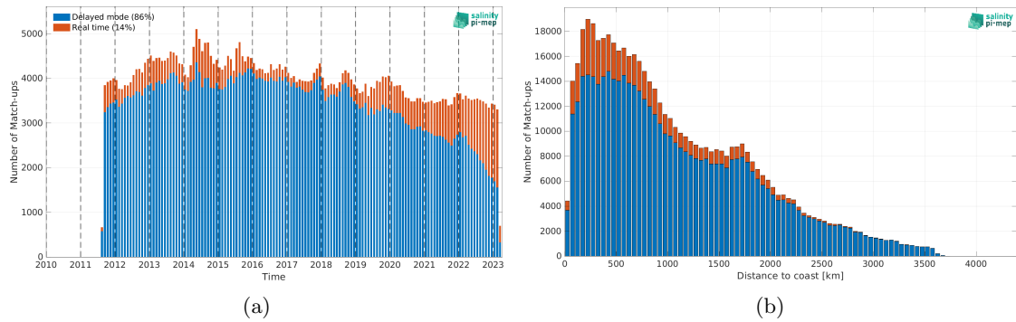
Figure 1: Number of match-ups between Argo and SMAP SSS L4 OI v2 - 7 Days (ESR) SSS as a function of time (a) and as function of the distance to coast (b) over the Pacific Ocean Pi-MEP region and for the full satellite product period.
