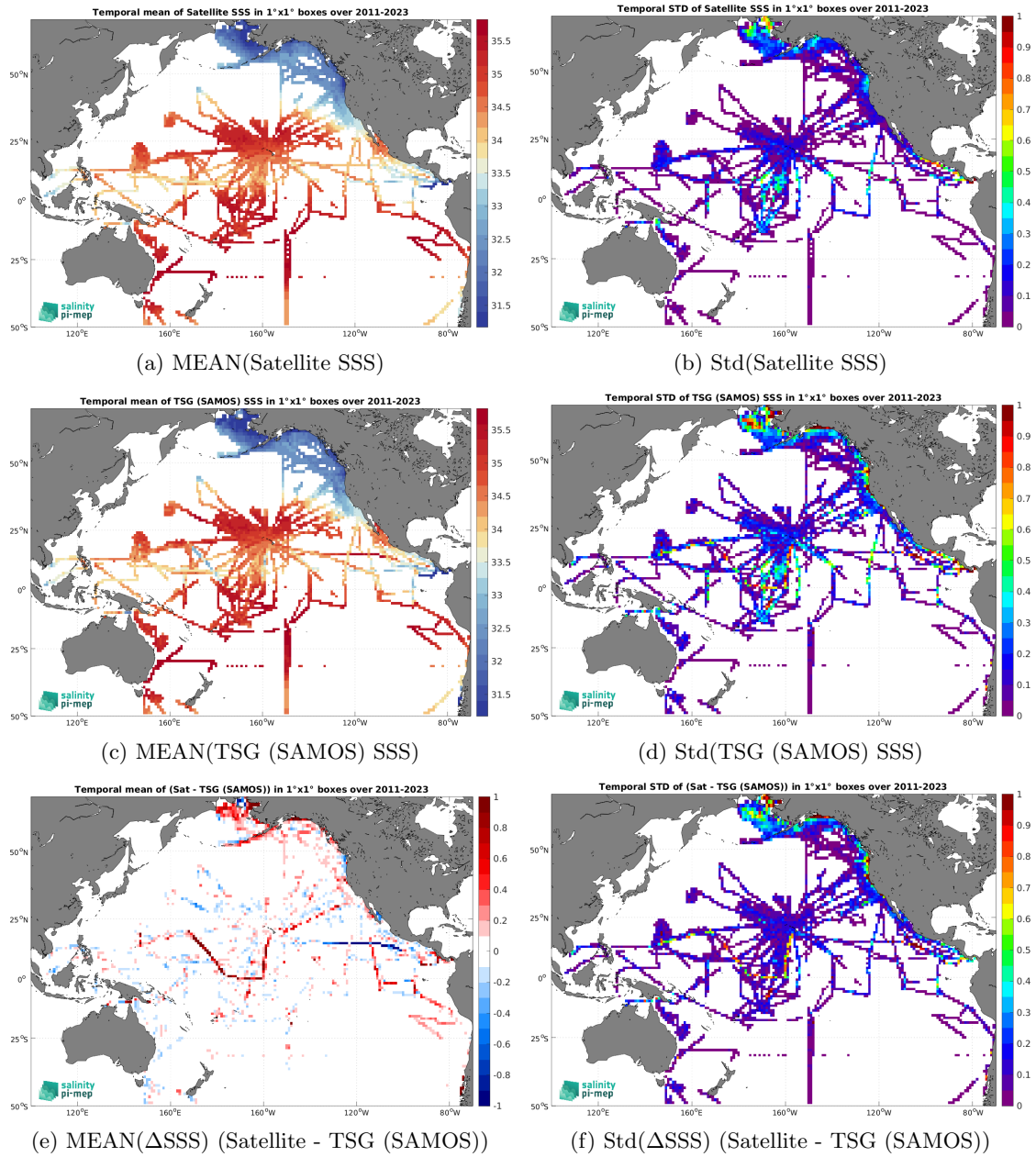
Figure 6: Temporal mean (left) and Std (right) of SSS from SMAP SSS L4 OI v2 - Monthly (IPRC) (top), TSG (SAMOS) (middle), and of \Delta SSS (Satellite - TSG (SAMOS)). Only match-up pairs are used to generate these maps.
