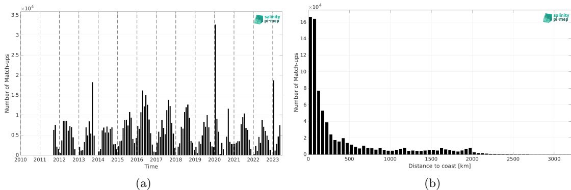
Figure 1: Number of match-ups between TSG (SAMOS) and SMAP SSS L4 OI v2 - Monthly (IPRC) SSS as a function of time (a) and as function of the distance to coast (b) over the Pacific Ocean Pi-MEP region and for the full satellite product period.
