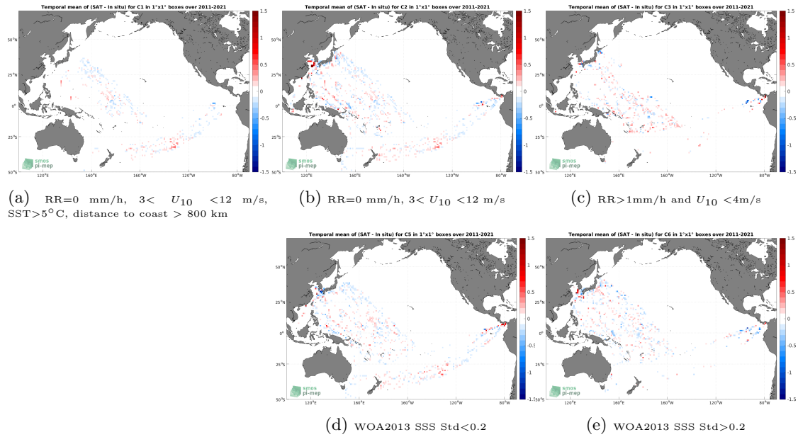
Figure 12: Temporal mean gridded over spatial boxes of size 1^\circ \times 1^\circ of \Delta SSS (SMAP SSS L4 OI v2 - Monthly (IPRC) - TSG (LEGOS-DM)) for 5 different subdatasets corresponding to:RR=0 mm/h, 3 < U_{10} < 12 m/s, SST >5^\circ C, distance to coast > 800 km (a), RR=0 mm/h, 3 < U_{10} < 12 m/s (b), RR >1 mm/h and U_{10} < 4 m/s (c), WOA2013 SSS Std <0.2 (d), WOA2013 SSS Std >0.2 (e).
