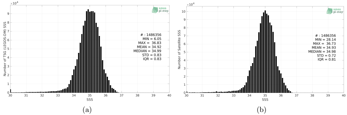
Figure 2: Histograms of SSS from TSG (LEGOS-DM) (a) and SMAP SSS L4 OI v2 - Monthly (IPRC) (b) considering all match-up pairs per bins of 0.1 over the Pacific Ocean Pi-MEP region and for the full satellite product period.
