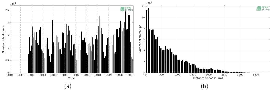
Figure 1: Number of match-ups between TSG (LEGOS-DM) and SMAP SSS L4 OI v2 - Monthly (IPRC) SSS as a function of time (a) and as function of the distance to coast (b) over the Pacific Ocean Pi-MEP region and for the full satellite product period.
