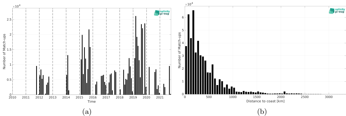
Figure 1: Number of match-ups between TSG (GOSUD-Research-vessel) and SMAP SSS L4 OI v2 - Monthly (IPRC) SSS as a function of time (a) and as function of the distance to coast (b) over the Pacific Ocean Pi-MEP region and for the full satellite product period.
