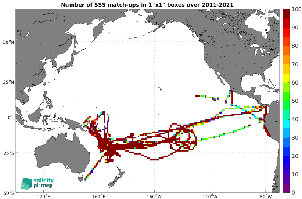
Figure 4: Number of SSS match-ups between TSG (GOSUD-Research-vessel) SSS and the SMAP SSS L4 OI v2 - Monthly (IPRC) SSS product for the Pacific Ocean Pi-MEP region over 1^\circ \times 1^\circ boxes and for the full satellite product period.
