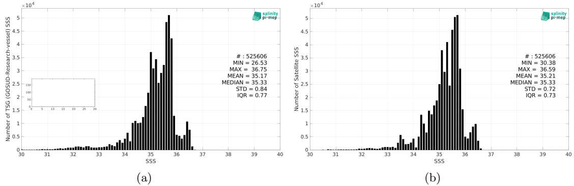
Figure 2: Histograms of SSS from TSG (GOSUD-Research-vessel) (a) and SMAP SSS L4 OI v2 - Monthly (IPRC) (b) considering all match-up pairs per bins of 0.1 over the Pacific Ocean Pi-MEP region and for the full satellite product period.
