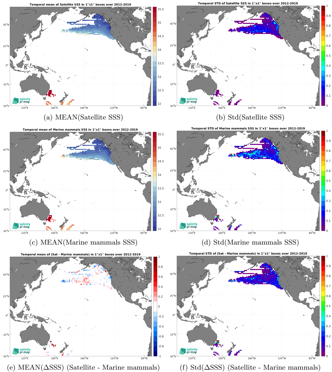
Figure 6: Temporal mean (left) and Std (right) of SSS from SMAP SSS L4 OI v2 - Monthly (IPRC) (top), Marine mammals (middle), and of \Delta SSS (Satellite - Marine mammals). Only match-up pairs are used to generate these maps.
