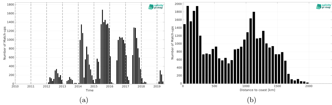
Figure 1: Number of match-ups between Marine mammals and SMAP SSS L4 OI v2 - Monthly (IPRC) SSS as a function of time (a) and as function of the distance to coast (b) over the Pacific Ocean Pi-MEP region and for the full satellite product period.
