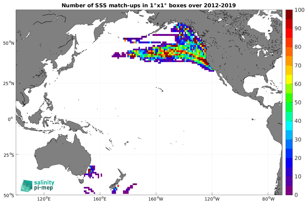
Figure 4: Number of SSS match-ups between Marine mammals SSS and the SMAP SSS L4 OI v2 - Monthly (IPRC) SSS product for the Pacific Ocean Pi-MEP region over 1^\circ \times 1^\circ boxes and for the full satellite product period.
