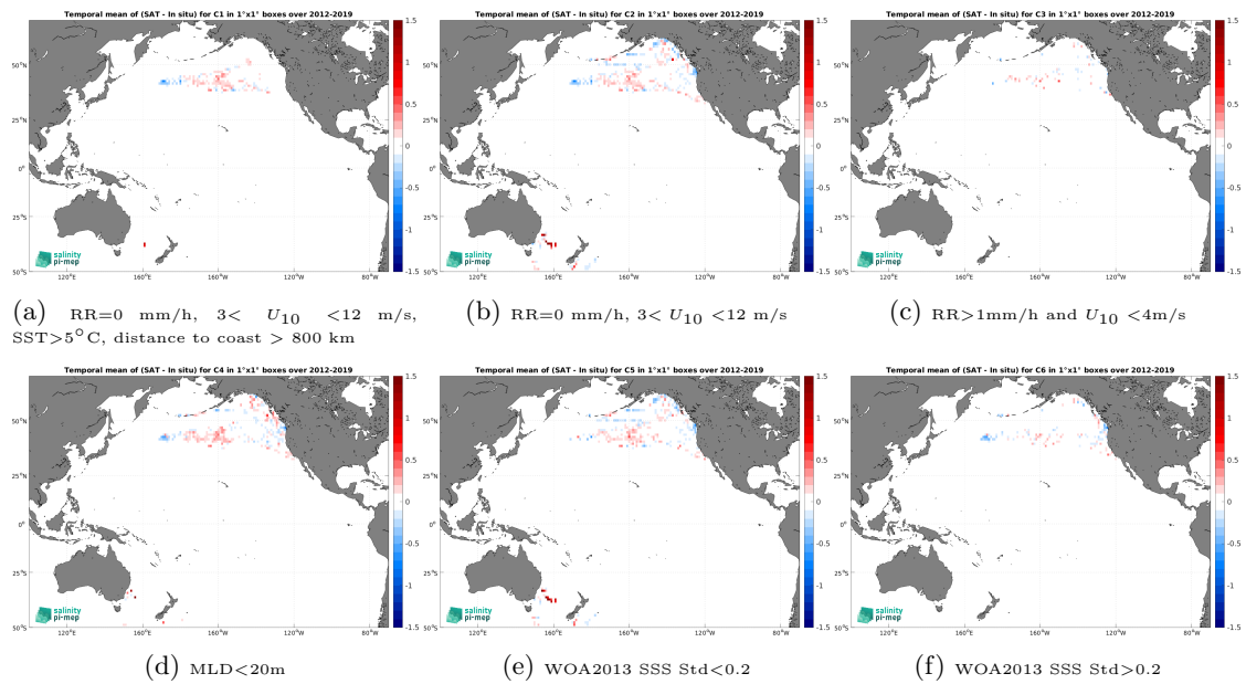
Figure 12: Temporal mean gridded over spatial boxes of size 1^\circ \times 1^\circ of \Delta SSS (SMAP SSS L4 OI v2 - Monthly (IPRC) - Marine mammals) for 6 different subdatasets corresponding to:RR=0 mm/h, 3 < U_{10} < 12 m/s, SST > 5^\circ\text{C} , distance to coast > 800 km (a), RR=0 mm/h, 3 < U_{10} < 12 m/s (b), RR > 1 mm/h and U_{10} < 4 m/s (c),MLD < 20 m (d),WOA2013 SSS Std < 0.2 (e),WOA2013 SSS Std > 0.2 (f).
