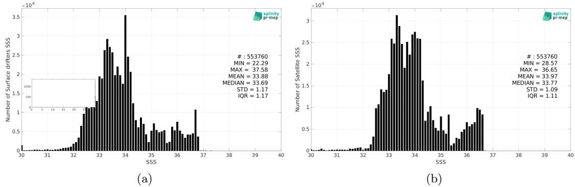
Figure 2: Histograms of SSS from Surface drifters (a) and SMAP SSS L4 OI v2 - Monthly (IPRC) (b) considering all match-up pairs per bins of 0.1 over the Pacific Ocean Pi-MEP region and for the full satellite product period.
