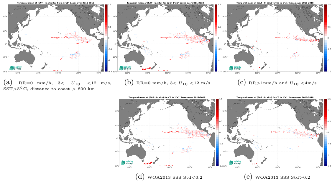
Figure 11: Temporal mean gridded over spatial boxes of size 1^\circ \times 1^\circ of \Delta\text{SSS} (SMAP SSS L4 OI v2 - Monthly (IPRC) - Surface drifters) for 5 different subdatasets corresponding to:RR=0 mm/h, 3 < U_{10} < 12 m/s, SST >5^\circ\text{C} , distance to coast > 800 km (a), RR=0 mm/h, 3 < U_{10} < 12 m/s (b), RR >1 mm/h and U_{10} < 4 m/s (c), WOA2013 SSS Std <0.2 (d), WOA2013 SSS Std >0.2 (e).
