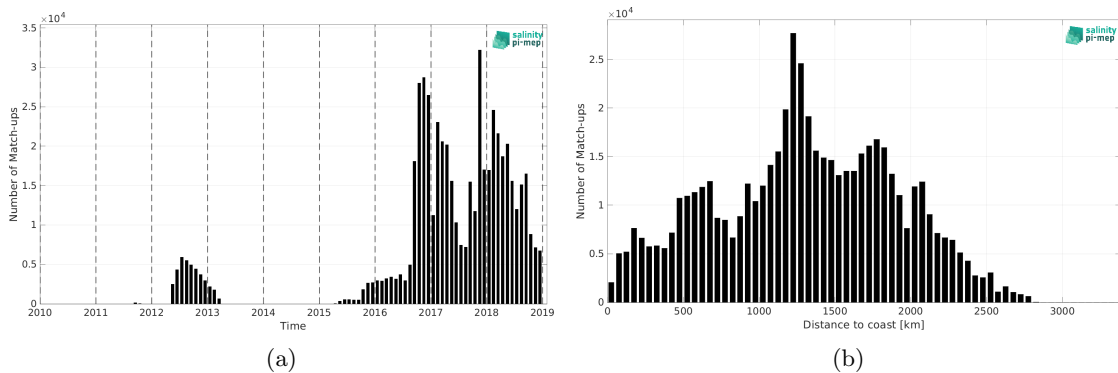
Figure 1: Number of match-ups between Surface drifters and SMAP SSS L4 OI v2 - Monthly (IPRC) SSS as a function of time (a) and as function of the distance to coast (b) over the Pacific Ocean Pi-MEP region and for the full satellite product period.
