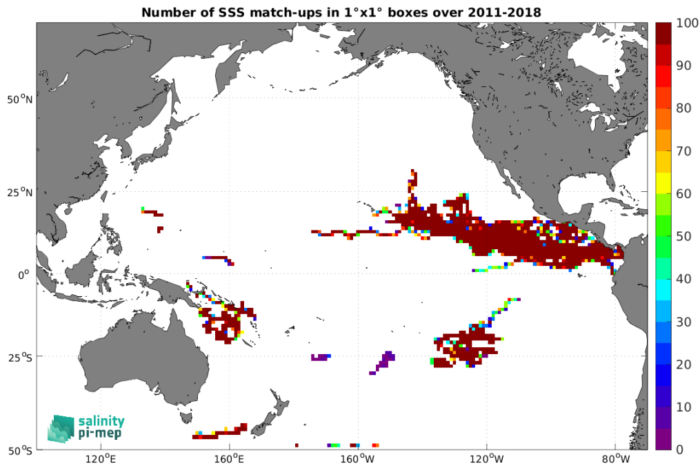
Figure 3: Number of SSS match-ups between Surface drifters SSS and the SMAP SSS L4 OI v2 - Monthly (IPRC) SSS product for the Pacific Ocean Pi-MEP region over 1^\circ \times 1^\circ boxes and for the full satellite product period.
