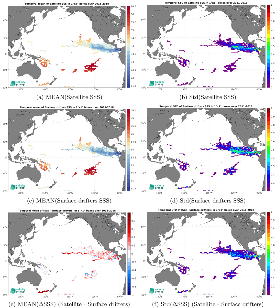
Figure 5: Temporal mean (left) and Std (right) of SSS from SMAP SSS L4 OI v2 - Monthly (IPRC) (top), Surface drifters (middle), and of \Delta SSS (Satellite - Surface drifters). Only match-up pairs are used to generate these maps.
