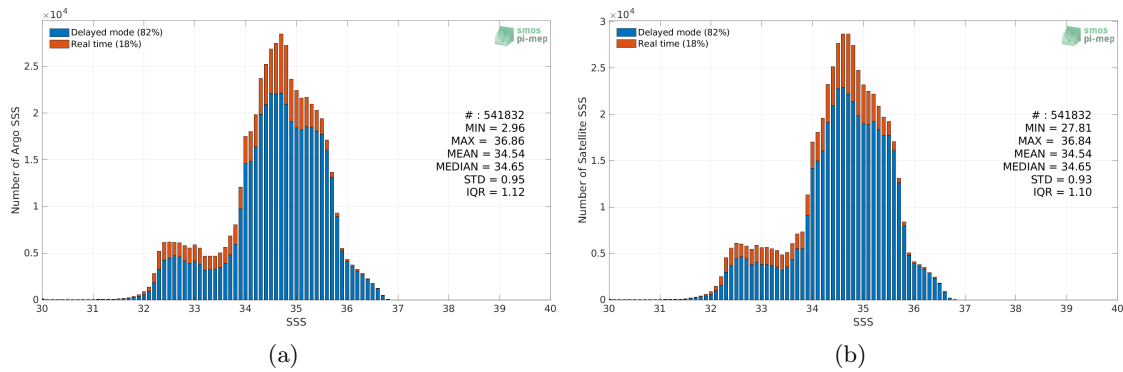
Figure 2: Histograms of SSS from Argo (a) and SMAP SSS L4 OI v2 - Monthly (IPRC) (b) considering all match-up pairs per bins of 0.1 over the Pacific Ocean Pi-MEP region and for the full satellite product period.
