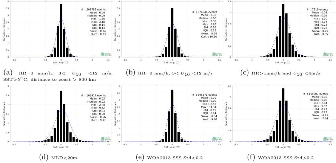
Figure 13: Normalized histogram of \Delta SSS (SMAP SSS L4 OI v2 - Monthly (IPRC) - Argo) for 6 different subdatasets corresponding to: RR=0 mm/h, 3 < U_{10} < 12 m/s, SST > 5°C, distance to coast > 800 km (a), RR=0 mm/h, 3 < U_{10} < 12 m/s (b), RR > 1mm/h and U_{10} < 4 m/s (c), MLD < 20m (d), WOA2013 SSS Std < 0.2 (e), WOA2013 SSS Std > 0.2 (f).
