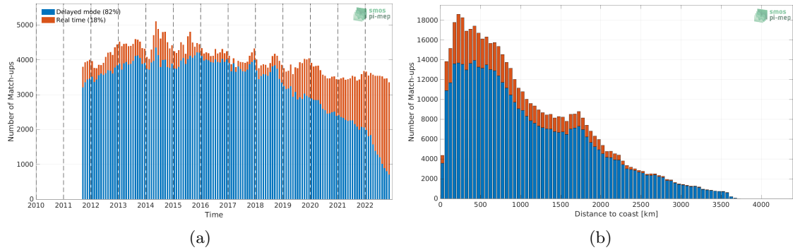
Figure 1: Number of match-ups between Argo and SMAP SSS L4 OI v2 - Monthly (IPRC) SSS as a function of time (a) and as function of the distance to coast (b) over the Pacific Ocean Pi-MEP region and for the full satellite product period.
