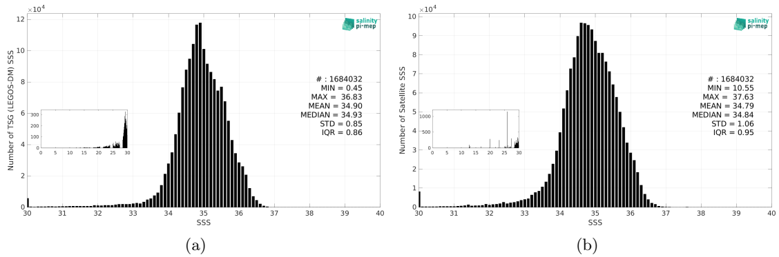
Figure 3: Histograms of SSS from TSG (LEGOS-DM) (a) and SMAP SSS L3 v6 - 8-Day running (RSS) (b) considering all match-up pairs per bins of 0.1 over the Pacific Ocean Pi-MEP region and for the full satellite product period.
