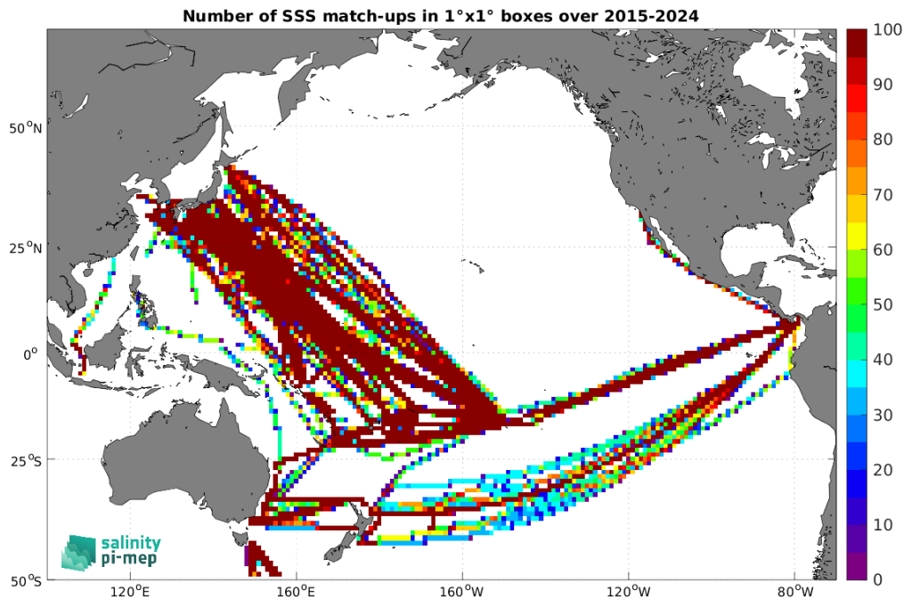
Figure 5: Number of SSS match-ups between TSG (LEGOS-DM) SSS and the SMAP SSS L3 v6 - 8-Day running (RSS) SSS product for the Pacific Ocean Pi-MEP region over 1^\circ \times 1^\circ boxes and for the full satellite product period.
