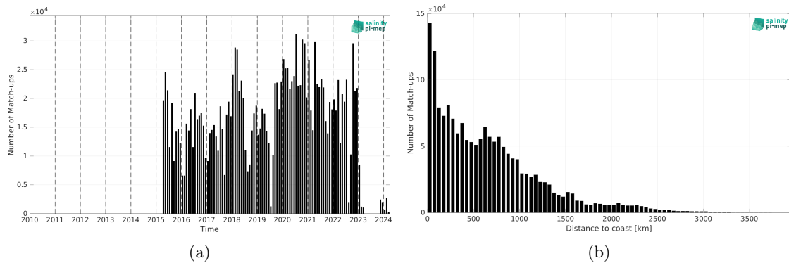
Figure 2: Number of match-ups between TSG (LEGOS-DM) and SMAP SSS L3 v6 - 8-Day running (RSS) SSS as a function of time (a) and as function of the distance to coast (b) over the Pacific Ocean Pi-MEP region and for the full satellite product period.
