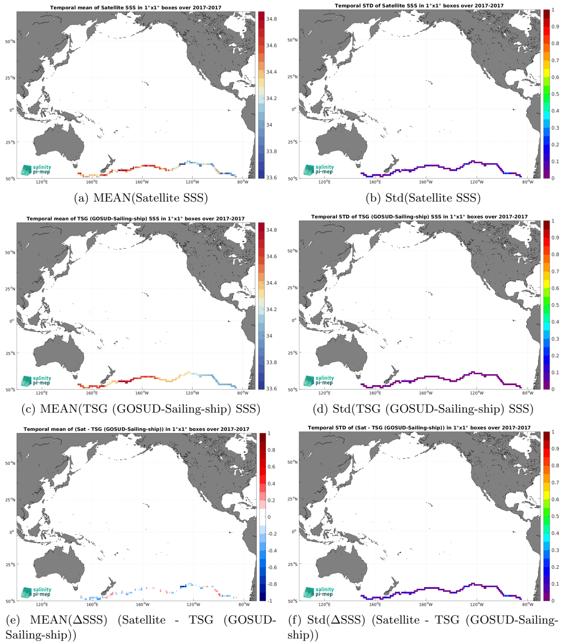
Figure 7: Temporal mean (left) and Std (right) of SSS from SMAP SSS L3 v6 - 8-Day running (RSS) (top), TSG (GOSUD-Sailing-ship) (middle), and of \Delta SSS (Satellite - TSG (GOSUD-Sailing-ship)). Only match-up pairs are used to generate these maps.
