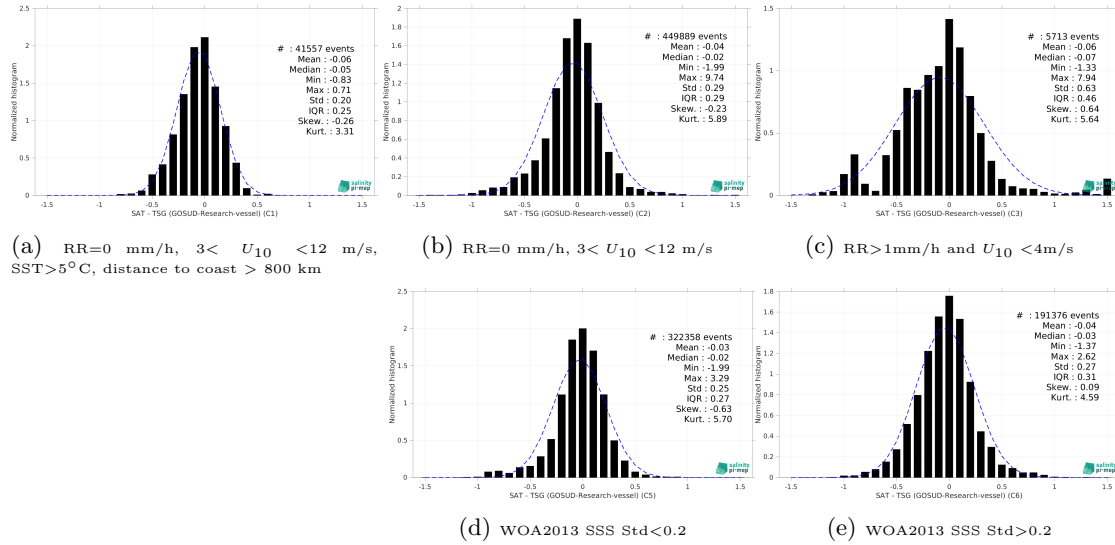
Figure 15: Normalized histogram of \Delta\text{SSS} (SMAP SSS L3 v6 - 8-Day running (RSS) - TSG (GOSUD-Research-vessel)) for 5 different subdatasets corresponding to: RR=0 mm/h, 3 < U_{10} < 12 m/s, SST>5°C, distance to coast > 800 km (a), RR=0 mm/h, 3 < U_{10} < 12 m/s (b), RR>1mm/h and U_{10} < 4 m/s (c), WOA2013 SSS Std<0.2 (d), WOA2013 SSS Std>0.2 (e).
