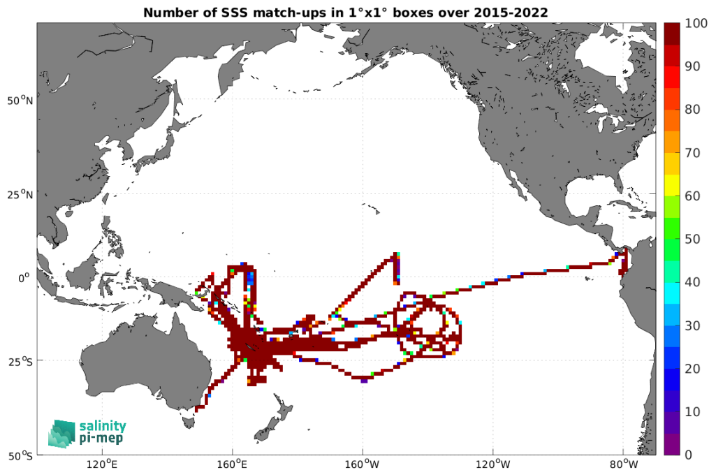
Figure 5: Number of SSS match-ups between TSG (GOSUD-Research-vessel) SSS and the SMAP SSS L3 v6 - 8-Day running (RSS) SSS product for the Pacific Ocean Pi-MEP region over 1^\circ \times 1^\circ boxes and for the full satellite product period.
