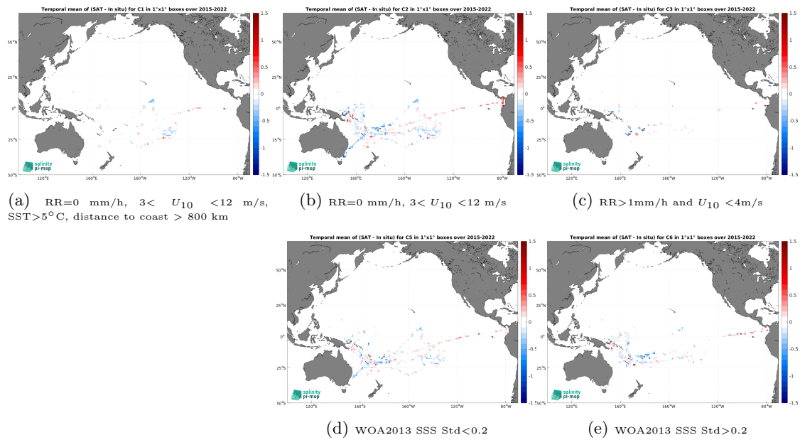
Figure 14: Temporal mean gridded over spatial boxes of size 1^\circ \times 1^\circ of \Delta SSS (SMAP SSS L3 v6 - 8-Day running (RSS) - TSG (GOSUD-Research-vessel)) for 5 different subdatasets corresponding to:RR=0 mm/h, 3 < U_{10} < 12 m/s, SST > 5^\circ\text{C} , distance to coast > 800 km (a), RR=0 mm/h, 3 < U_{10} < 12 m/s (b), RR > 1 mm/h and U_{10} < 4 m/s (c), WOA2013 SSS Std < 0.2 (d), WOA2013 SSS Std > 0.2 (e).
