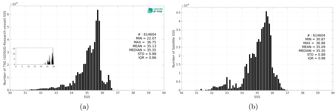
Figure 3: Histograms of SSS from TSG (GOSUD-Research-vessel) (a) and SMAP SSS L3 v6 - 8-Day running (RSS) (b) considering all match-up pairs per bins of 0.1 over the Pacific Ocean Pi-MEP region and for the full satellite product period.
