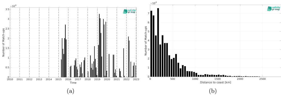
Figure 2: Number of match-ups between TSG (GOSUD-Research-vessel) and SMAP SSS L3 v6 - 8-Day running (RSS) SSS as a function of time (a) and as function of the distance to coast (b) over the Pacific Ocean Pi-MEP region and for the full satellite product period.
