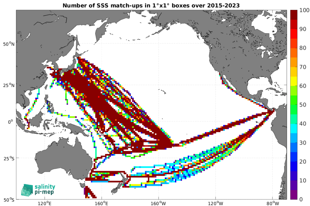
Figure 5: Number of SSS match-ups between TSG (LEGOS-DM) SSS and the SMAP SSS L3 v6 - Monthly (RSS) SSS product for the Pacific Ocean Pi-MEP region over 1^\circ \times 1^\circ boxes and for the full satellite product period.
