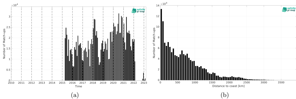
Figure 2: Number of match-ups between TSG (LEGOS-DM) and SMAP SSS L3 v6 - Monthly (RSS) SSS as a function of time (a) and as function of the distance to coast (b) over the Pacific Ocean Pi-MEP region and for the full satellite product period.
