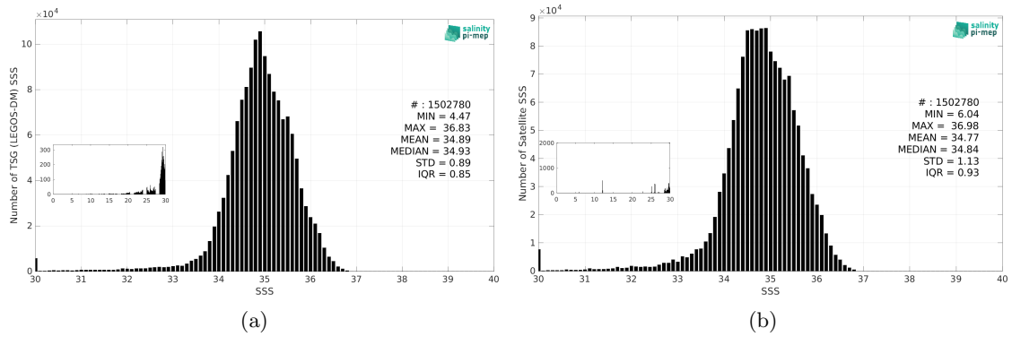
Figure 3: Histograms of SSS from TSG (LEGOS-DM) (a) and SMAP SSS L3 v6 - Monthly (RSS) (b) considering all match-up pairs per bins of 0.1 over the Pacific Ocean Pi-MEP region and for the full satellite product period.
