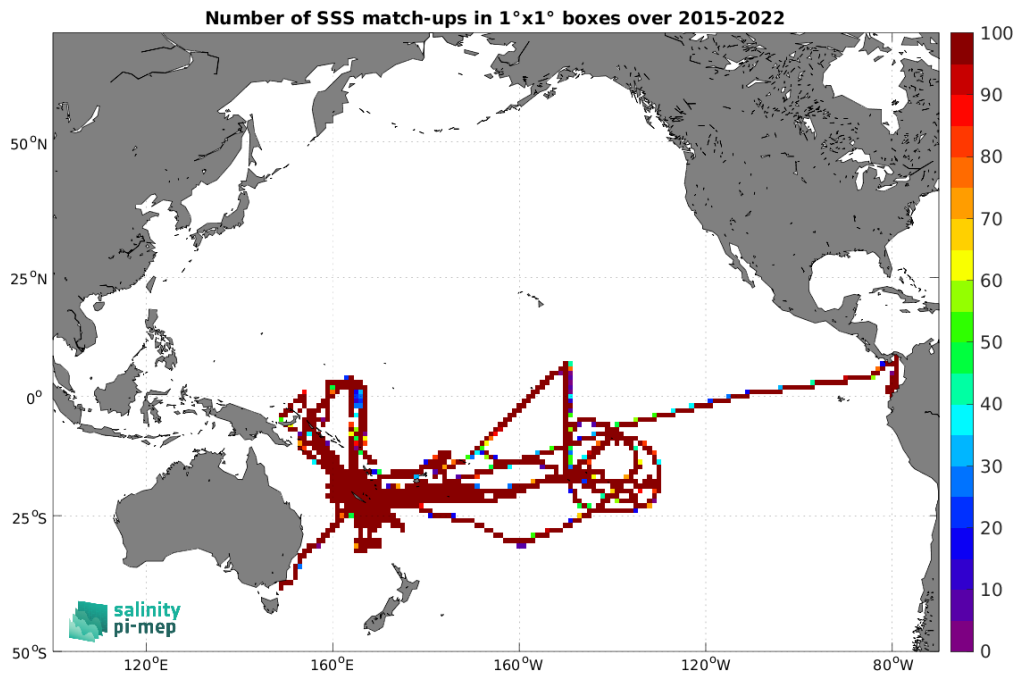
Figure 5: Number of SSS match-ups between TSG (GOSUD-Research-vessel) SSS and the SMAP SSS L3 v6 - Monthly (RSS) SSS product for the Pacific Ocean Pi-MEP region over 1^\circ \times 1^\circ boxes and for the full satellite product period.
