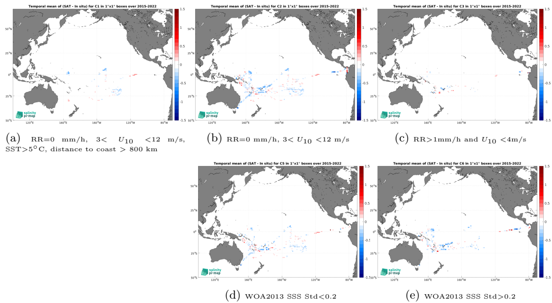
Figure 14: Temporal mean gridded over spatial boxes of size 1^\circ \times 1^\circ of \Delta SSS (SMAP SSS L3 v6 - Monthly (RSS) - TSG (GOSUD-Research-vessel)) for 5 different subdatasets corresponding to: RR=0 mm/h, 3 < U_{10} < 12 m/s, SST > 5^\circ\text{C} , distance to coast > 800 km (a), RR=0 mm/h, 3 < U_{10} < 12 m/s (b), RR > 1 mm/h and U_{10} < 4 m/s (c), WOA2013 SSS Std < 0.2 (d), WOA2013 SSS Std > 0.2 (e).
