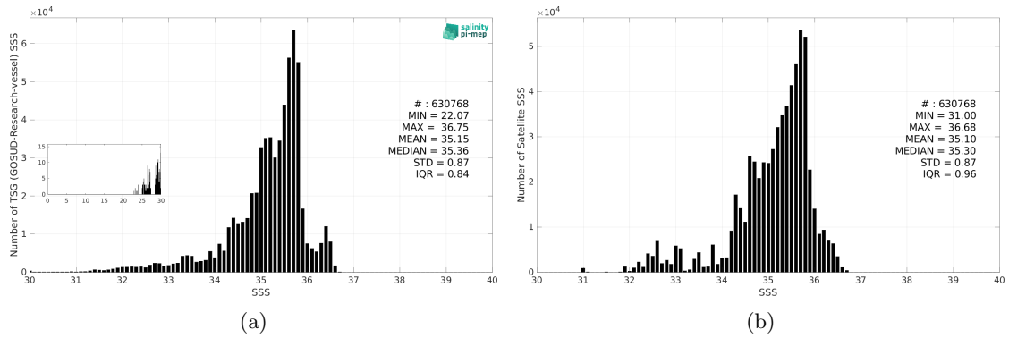
Figure 3: Histograms of SSS from TSG (GOSUD-Research-vessel) (a) and SMAP SSS L3 v6 - Monthly (RSS) (b) considering all match-up pairs per bins of 0.1 over the Pacific Ocean Pi-MEP region and for the full satellite product period.
