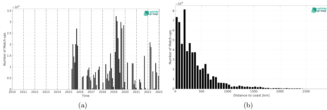
Figure 2: Number of match-ups between TSG (GOSUD-Research-vessel) and SMAP SSS L3 v6 - Monthly (RSS) SSS as a function of time (a) and as function of the distance to coast (b) over the Pacific Ocean Pi-MEP region and for the full satellite product period.
