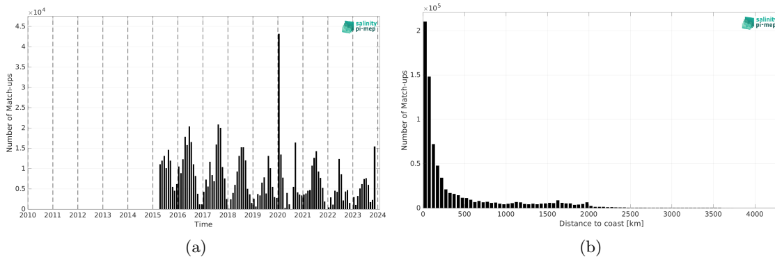
Figure 2: Number of match-ups between TSG (SAMOS) and SMAP SSS L3 v5.3 - 8-Day running (RSS) SSS as a function of time (a) and as function of the distance to coast (b) over the Pacific Ocean Pi-MEP region and for the full satellite product period.
