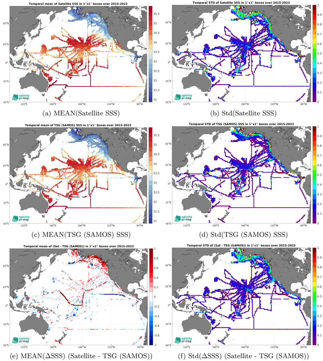
Figure 7: Temporal mean (left) and Std (right) of SSS from SMAP SSS L3 v5.3 - 8-Day running (RSS) (top), TSG (SAMOS) (middle), and of \Delta SSS (Satellite - TSG (SAMOS)). Only match-up pairs are used to generate these maps.
