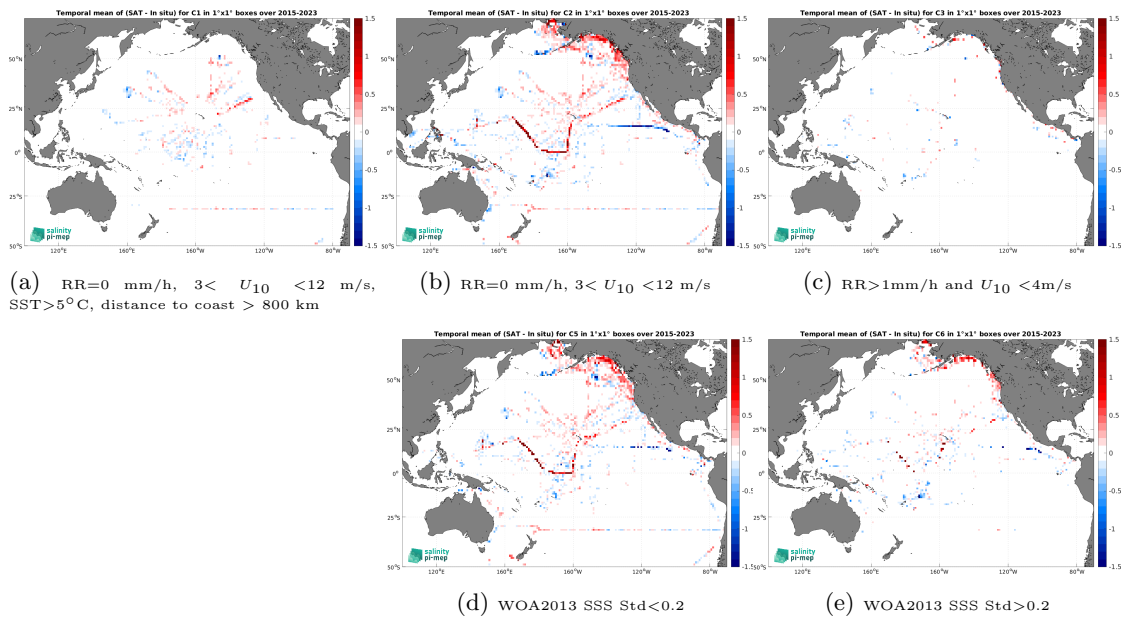
Figure 14: Temporal mean gridded over spatial boxes of size 1^\circ \times 1^\circ of \Delta SSS (SMAP SSS L3 v5.3 - 8-Day running (RSS) - TSG (SAMOS)) for 5 different subdatasets corresponding to:RR=0 mm/h, 3 < U_{10} < 12 m/s, SST > 5^\circ C , distance to coast > 800 km (a), RR=0 mm/h, 3 < U_{10} < 12 m/s (b), RR>1mm/h and U_{10} < 4m/s (c), WOA2013 SSS Std<0.2 (d), WOA2013 SSS Std>0.2 (e).
