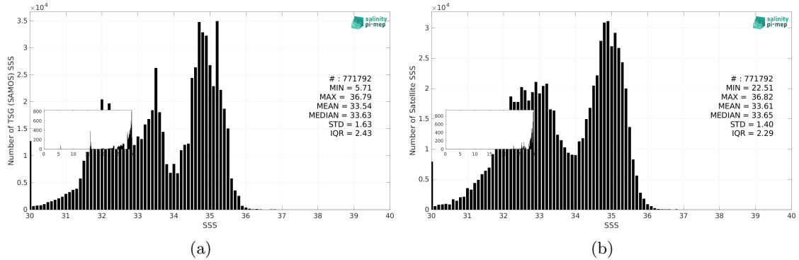
Figure 3: Histograms of SSS from TSG (SAMOS) (a) and SMAP SSS L3 v5.3 - 8-Day running (RSS) (b) considering all match-up pairs per bins of 0.1 over the Pacific Ocean Pi-MEP region and for the full satellite product period.
