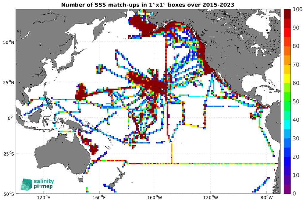
Figure 5: Number of SSS match-ups between TSG (SAMOS) SSS and the SMAP SSS L3 v5.3 - 8-Day running (RSS) SSS product for the Pacific Ocean Pi-MEP region over 1^\circ \times 1^\circ boxes and for the full satellite product period.
