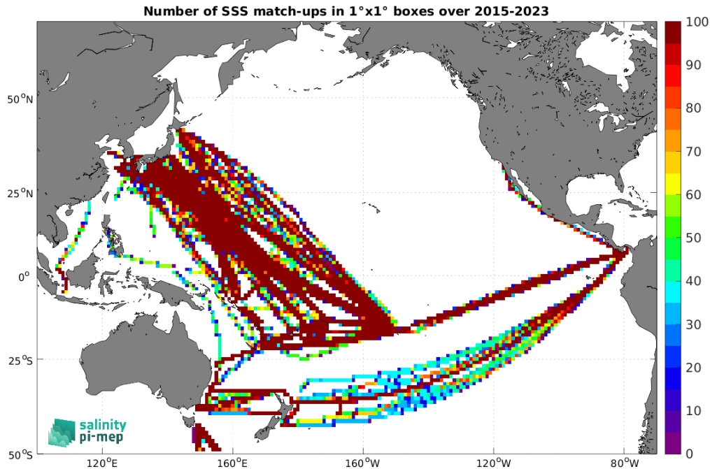
Figure 5: Number of SSS match-ups between TSG (LEGOS-DM) SSS and the SMAP SSS L3 v5.3 - 8-Day running (RSS) SSS product for the Pacific Ocean Pi-MEP region over 1^\circ \times 1^\circ boxes and for the full satellite product period.
