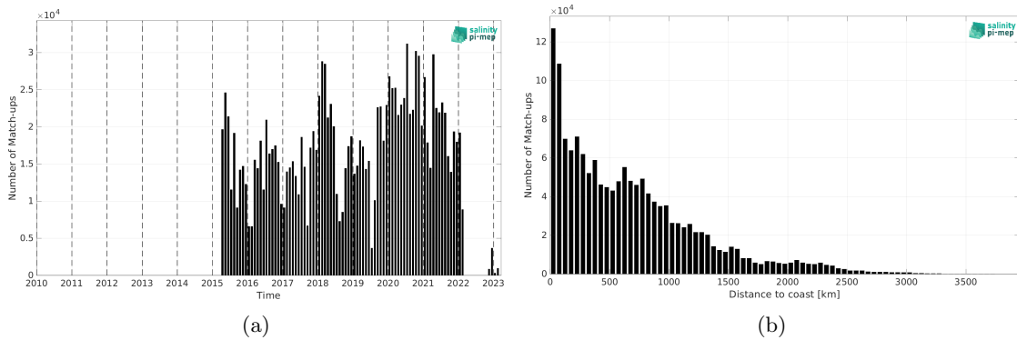
Figure 2: Number of match-ups between TSG (LEGOS-DM) and SMAP SSS L3 v5.3 - 8-Day running (RSS) SSS as a function of time (a) and as function of the distance to coast (b) over the Pacific Ocean Pi-MEP region and for the full satellite product period.
