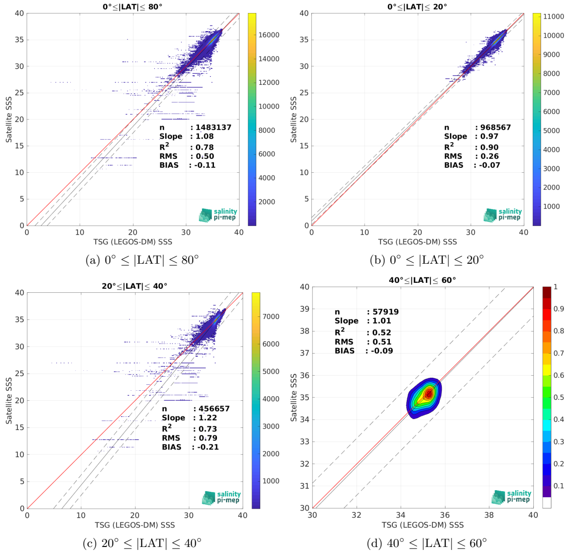
Figure 10: Contour maps of the concentration of SMAP SSS L3 v5.3 - 8-Day running (RSS) SSS (y-axis) versus TSG (LEGOS-DM) SSS (x-axis) at match-up pairs for different latitude bands. For each plot, the red line shows x=y . The black thin and dashed lines indicate a linear fit through the data cloud and the \pm 95\% confidence levels, respectively. The number match-up pairs n , the slope and R^2 coefficient of the linear fit, the root mean square (RMS) and the mean bias between satellite and in situ data are indicated for each latitude band in each plots.
