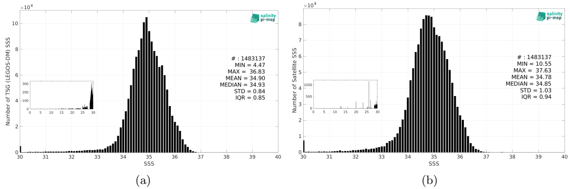
Figure 3: Histograms of SSS from TSG (LEGOS-DM) (a) and SMAP SSS L3 v5.3 - 8-Day running (RSS) (b) considering all match-up pairs per bins of 0.1 over the Pacific Ocean Pi-MEP region and for the full satellite product period.
