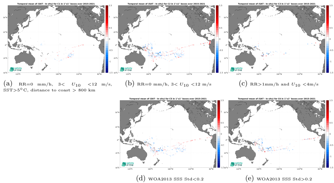
Figure 14: Temporal mean gridded over spatial boxes of size 1^\circ \times 1^\circ of \Delta SSS (SMAP SSS L3 v5.3 - 8-Day running (RSS) - TSG (GOSUD-Research-vessel)) for 5 different subdatasets corresponding to:RR=0 mm/h, 3 < U_{10} < 12 m/s, SST >5^\circ\text{C} , distance to coast > 800 km (a), RR=0 mm/h, 3 < U_{10} < 12 m/s (b), RR >1 mm/h and U_{10} < 4 m/s (c), WOA2013 SSS Std <0.2 (d), WOA2013 SSS Std >0.2 (e).
