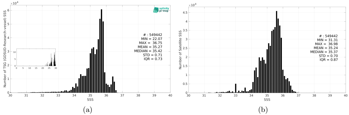
Figure 3: Histograms of SSS from TSG (GOSUD-Research-vessel) (a) and SMAP SSS L3 v5.3 - 8-Day running (RSS) (b) considering all match-up pairs per bins of 0.1 over the Pacific Ocean Pi-MEP region and for the full satellite product period.
