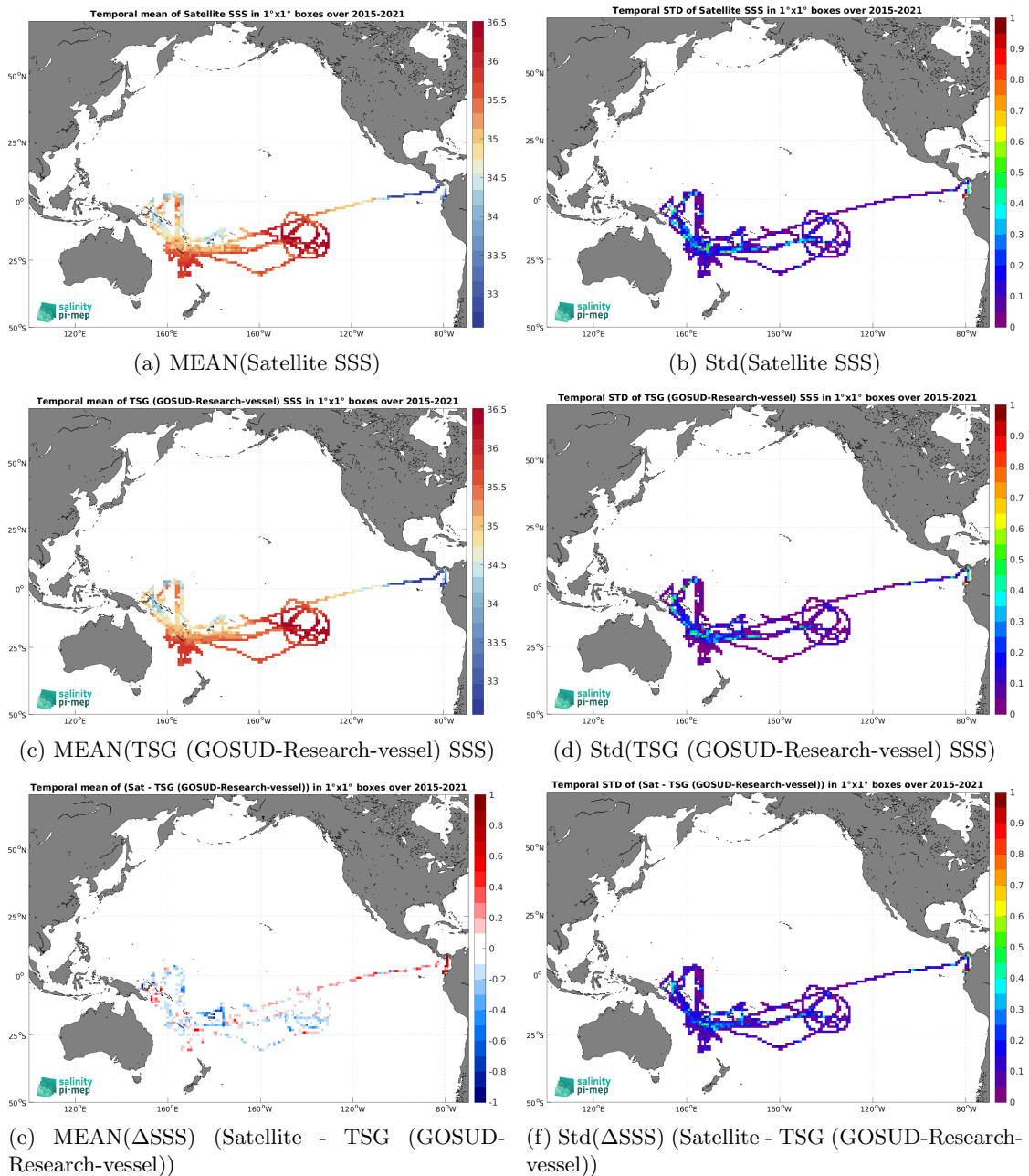
Figure 7: Temporal mean (left) and Std (right) of SSS from SMAP SSS L3 v5.3 - 8-Day running (RSS) (top), TSG (GOSUD-Research-vessel) (middle), and of \Delta SSS (Satellite - TSG (GOSUD-Research-vessel)). Only match-up pairs are used to generate these maps.
