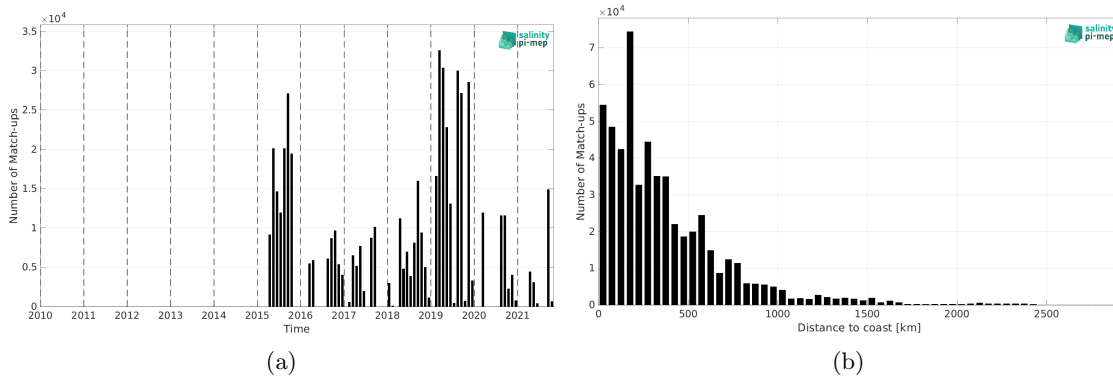
Figure 2: Number of match-ups between TSG (GOSUD-Research-vessel) and SMAP SSS L3 v5.3 - 8-Day running (RSS) SSS as a function of time (a) and as function of the distance to coast (b) over the Pacific Ocean Pi-MEP region and for the full satellite product period.
