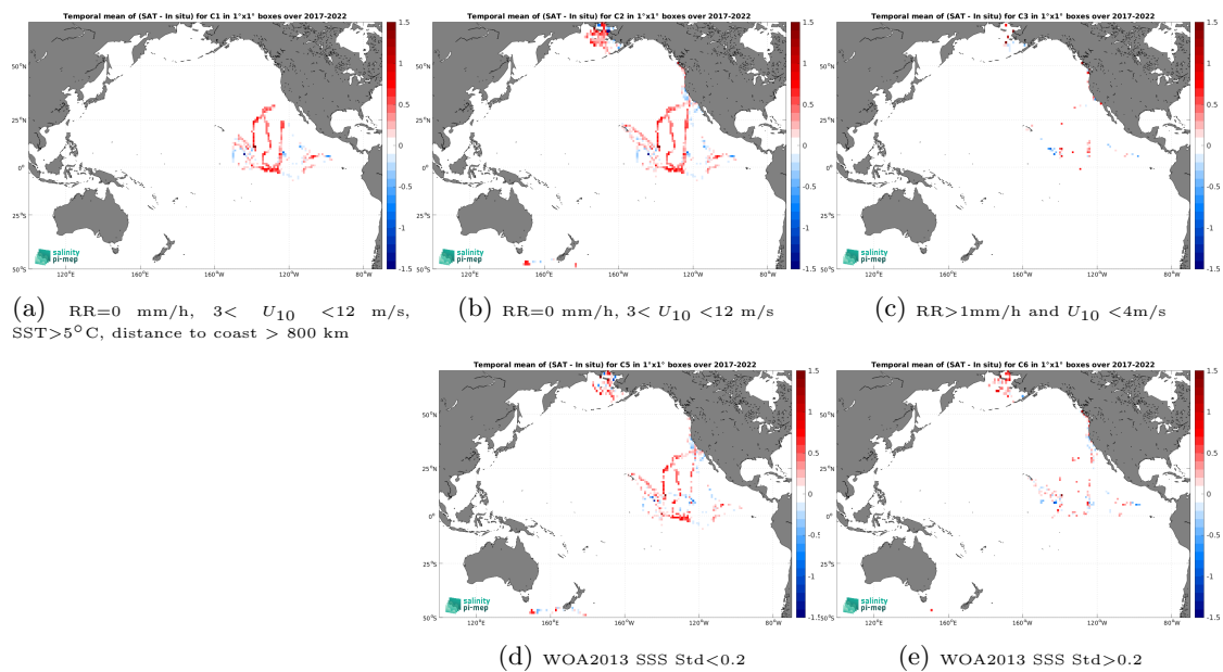
Figure 14: Temporal mean gridded over spatial boxes of size 1^\circ \times 1^\circ of \Delta SSS (SMAP SSS L3 v5.3 - 8-Day running (RSS) - Sairdrone) for 5 different subdatasets corresponding to:RR=0 mm/h, 3 < U_{10} < 12 m/s, SST > 5^\circ\text{C} , distance to coast > 800 km (a), RR=0 mm/h, 3 < U_{10} < 12 m/s (b), RR > 1 mm/h and U_{10} < 4 m/s (c), WOA2013 SSS Std < 0.2 (d), WOA2013 SSS Std > 0.2 (e).
