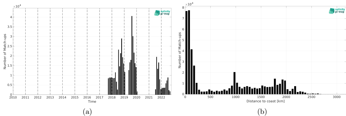
Figure 2: Number of match-ups between Saildrone and SMAP SSS L3 v5.3 - 8-Day running (RSS) SSS as a function of time (a) and as function of the distance to coast (b) over the Pacific Ocean Pi-MEP region and for the full satellite product period.
