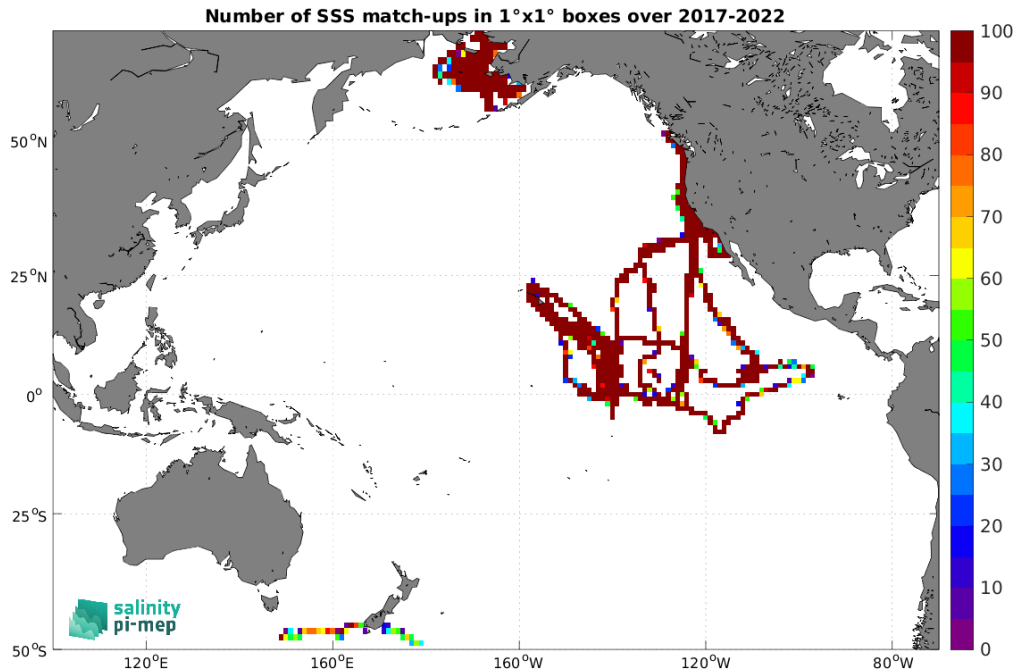
Figure 5: Number of SSS match-ups between Saildrone SSS and the SMAP SSS L3 v5.3 - 8-Day running (RSS) SSS product for the Pacific Ocean Pi-MEP region over 1^\circ \times 1^\circ boxes and for the full satellite product period.
