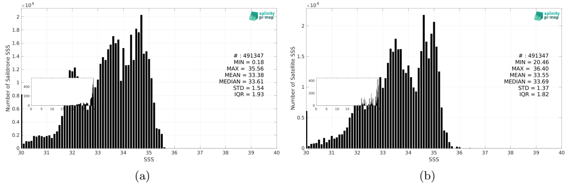
Figure 3: Histograms of SSS from Saildrone (a) and SMAP SSS L3 v5.3 - 8-Day running (RSS) (b) considering all match-up pairs per bins of 0.1 over the Pacific Ocean Pi-MEP region and for the full satellite product period.
