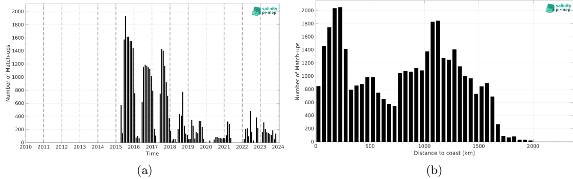
Figure 2: Number of match-ups between Marine mammals and SMAP SSS L3 v5.3 - 8-Day running (RSS) SSS as a function of time (a) and as function of the distance to coast (b) over the Pacific Ocean Pi-MEP region and for the full satellite product period.
