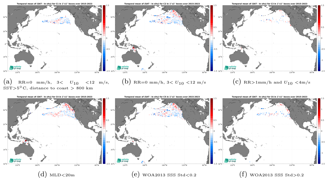
Figure 14: Temporal mean gridded over spatial boxes of size 1^\circ \times 1^\circ of \Delta SSS (SMAP SSS L3 v5.3 - 8-Day running (RSS) - Marine mammals) for 6 different subdatasets corresponding to:RR=0 mm/h, 3 < U_{10} < 12 m/s, SST >5^\circ C, distance to coast > 800 km (a), RR=0 mm/h, 3 < U_{10} < 12 m/s (b), RR >1 mm/h and U_{10} < 4 m/s (c),MLD <20 m (d),WOA2013 SSS Std <0.2 (e),WOA2013 SSS Std >0.2 (f).
