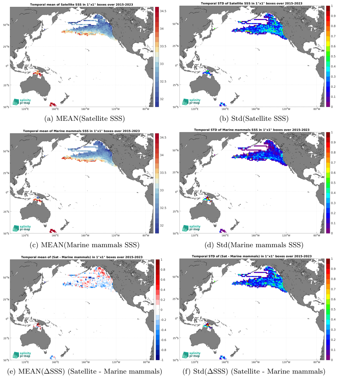
Figure 7: Temporal mean (left) and Std (right) of SSS from SMAP SSS L3 v5.3 - 8-Day running (RSS) (top), Marine mammals (middle), and of \Delta SSS (Satellite - Marine mammals). Only match-up pairs are used to generate these maps.
