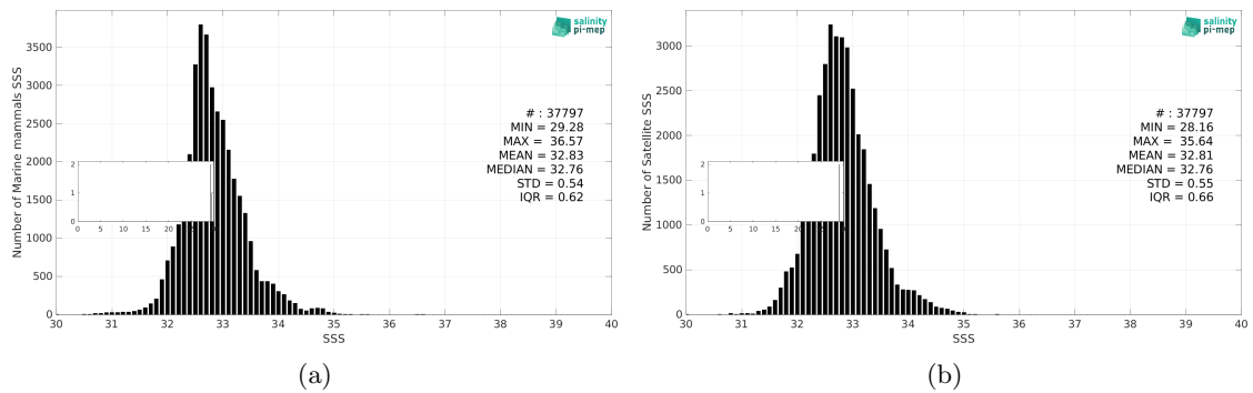
Figure 3: Histograms of SSS from Marine mammals (a) and SMAP SSS L3 v5.3 - 8-Day running (RSS) (b) considering all match-up pairs per bins of 0.1 over the Pacific Ocean Pi-MEP region and for the full satellite product period.
