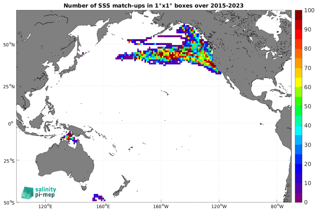
Figure 5: Number of SSS match-ups between Marine mammals SSS and the SMAP SSS L3 v5.3 - 8-Day running (RSS) SSS product for the Pacific Ocean Pi-MEP region over 1^\circ \times 1^\circ boxes and for the full satellite product period.
